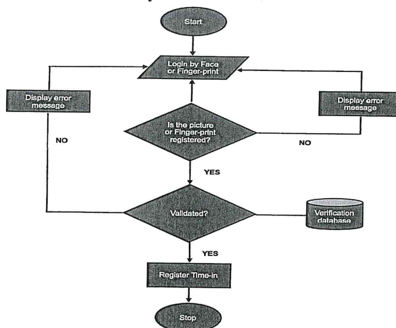
Fig. 1: Illustration of the Biometric System Flowchart
