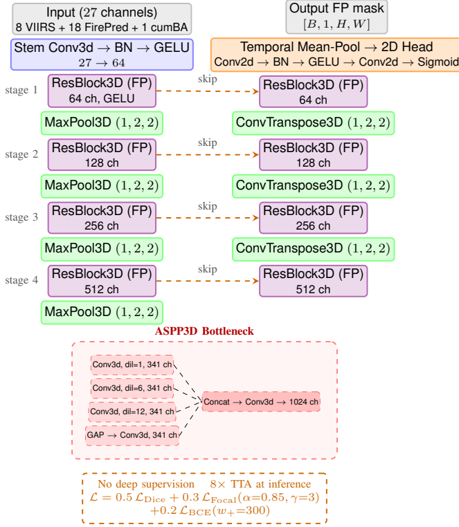
Fig. 3: SpaSE-UNet3D FP variant. The encoder takes a 27-channel input combining VIIRS, FirePred auxiliary bands, and a cumulative burned-area mask. The bottleneck is replaced with an ASPP3D module that aggregates multi-scale context via parallel dilated convolutions and a global average pool. The final head collapses the temporal dimension via a mean-pool and applies a 2D convolutional head to produce a single-day FP mask. No deep supervision is used; 8\times test-time augmentation is applied at inference.
