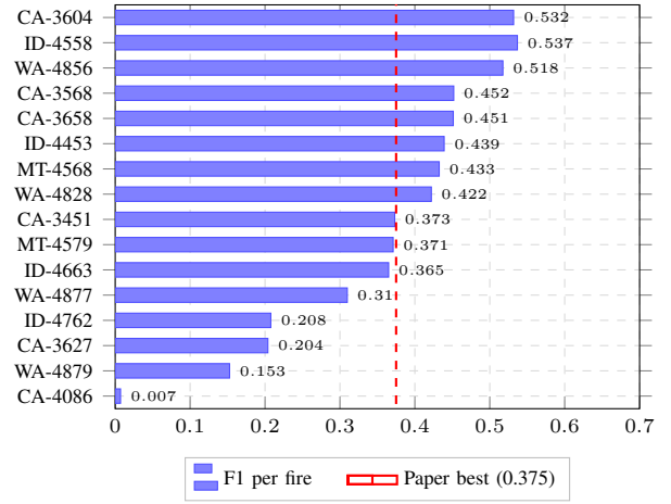
Fig. 6: Per-fire test F1 for SpaSE-UNet3D on the 16 usable US_2021 fires (sorted by F1). Eight fires with near-zero progression signal are excluded as discussed in Section IV. Red dashed line: best paper baseline (0.375).
