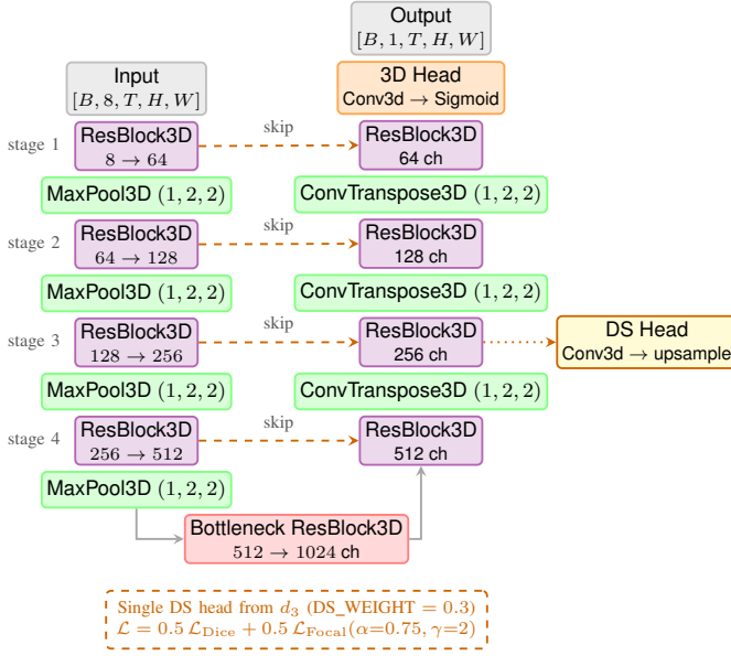
Fig. 2: SpaSE-UNet3D AF variant. The encoder (left column) takes an 8-channel VIIRS input and downsamples spatially through four ResBlock3D stages with channels [64, 128, 256, 512]. A single ResBlock3D bottleneck widens to 1024 channels. The decoder (right column) mirrors the encoder with channel concatenation at every skip. A 3D head produces per-day fire masks. Deep supervision is applied at every decoder stage.
