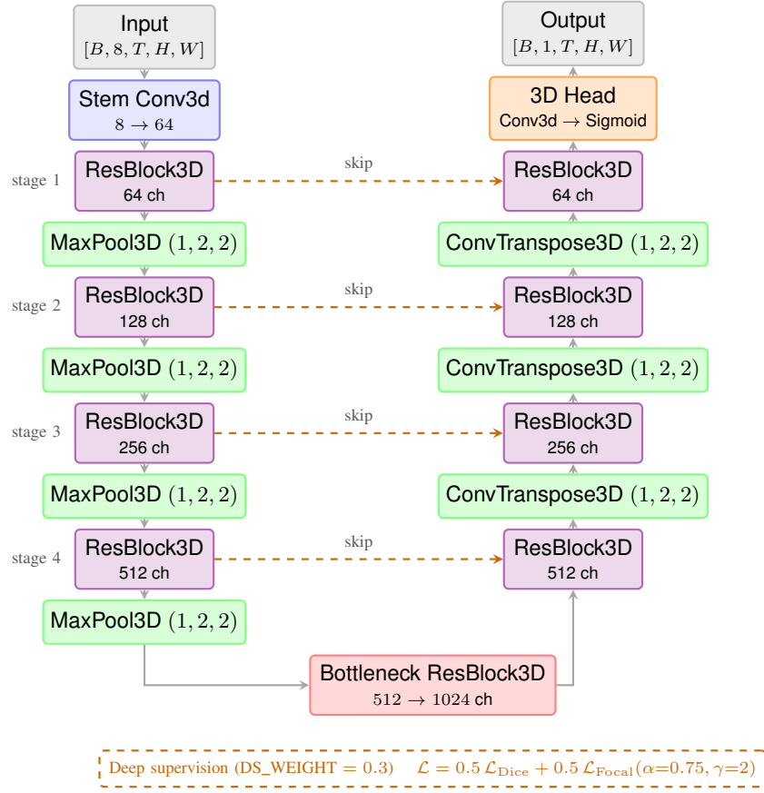
Fig. 2: SpaSE-UNet3D AF variant. The encoder (left column) takes an 8-channel VIIRS input and downsamples spatially through four ResBlock3D stages with channels [64, 128, 256, 512] . A single ResBlock3D bottleneck widens to 1024 channels. The decoder (right column) mirrors the encoder with channel concatenation at every skip. A 3D head produces per-day fire masks. Deep supervision is applied at every decoder stage.
