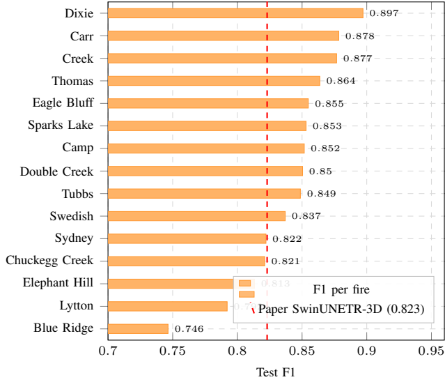
Fig. 6: Per-fire test F1 for SpaSE-UNet3D at TS = 2 on the audited AF test set (15 fires, sorted by F1). Red dashed line: SwinUNETR-3D paper baseline.
