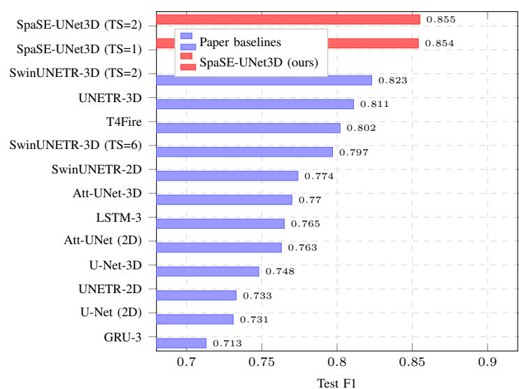
Fig. 8: Active Fire benchmark comparison vs. the 12 paper baselines [2]. Our SpaSE-UNet3D results (TS = 1 and TS = 2) shown in red.
