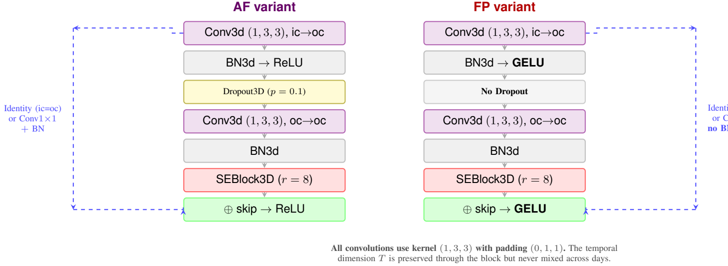
Fig. 1: Internal structure of the ResBlock3D used in both SpaSE-UNet3D variants. Both blocks share spatial-only (1, 3, 3) convolutions and SE channel attention. The AF variant (left) uses ReLU activations and Dropout3D for regularisation; the FP variant (right) uses GELU and removes Dropout, which empirically hurt convergence on the smaller, sparser FP training set. The skip path either passes the input unchanged (when ic = oc ) or applies a 1 \times 1 \times 1 projection convolution.
