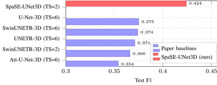
Fig. 10: Fire Progression benchmark comparison. Our SpaSE-UNet3D at TS = 2 shown in red, alongside the five paper baselines [2] at TS = 2 and TS = 6.
