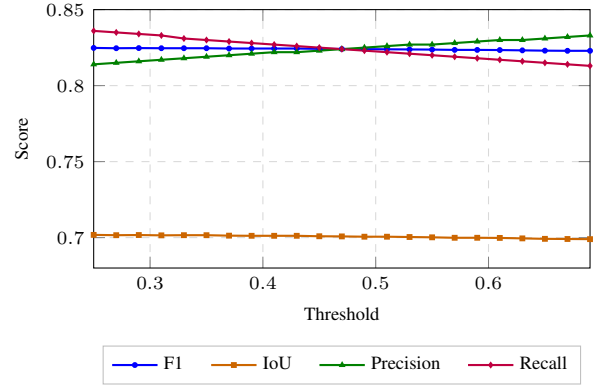
Fig. 4: Active Fire validation threshold sweep at TS = 2. F1 and IoU are nearly flat across [0.25, 0.69] ; precision and recall trade off symmetrically around 0.50. The model is robust to threshold selection.
