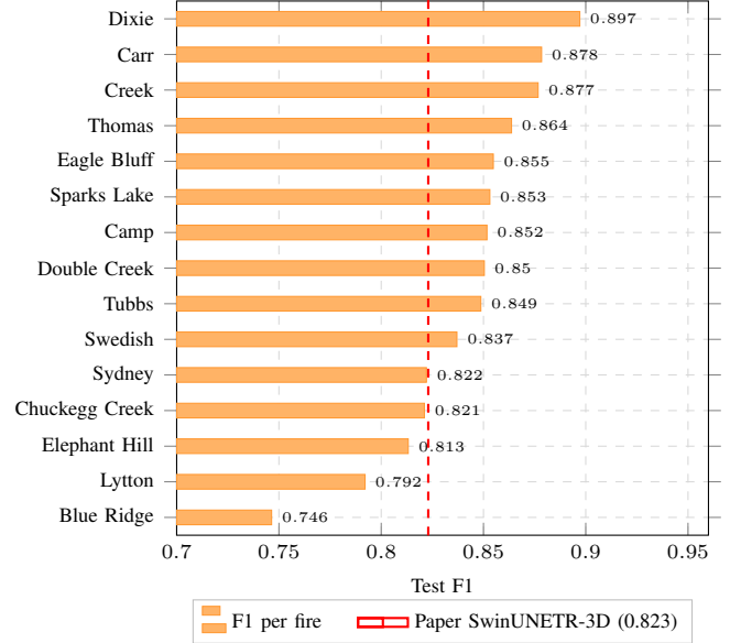
Fig. 4: Per-fire test F1 for SpaSE-UNet3D at TS = 2 on the audited AF test set (15 fires, sorted by F1). Red dashed line: SwinUNETR-3D paper baseline.
