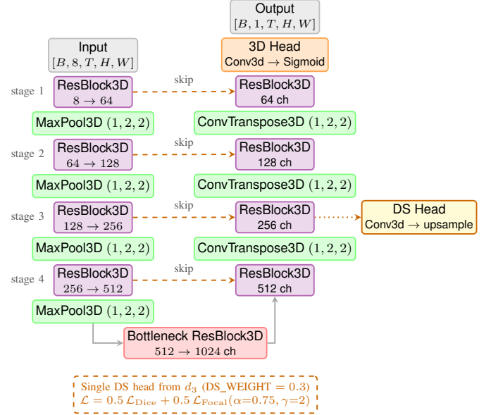
Fig. 2: SpaSE-UNet3D AF variant. The encoder (left column) takes an 8-channel VIIRS input and downsamples spatially through four ResBlock3D stages with channels [64, 128, 256, 512]. A single ResBlock3D bottleneck widens to 1024 channels. The decoder (right column) mirrors the encoder with channel concatenation at every skip. A 3D head produces per-day fire masks. Deep supervision is applied at every decoder stage.
