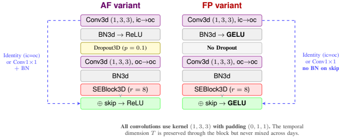
Fig. 1: Internal structure of the ResBlock3D used in both SpaSE-UNet3D variants. Both blocks share spatial-only (1, 3, 3) convolutions and SE channel attention. The AF variant (left) uses ReLU activations and Dropout3D for regularisation; the FP variant (right) uses GELU and removes Dropout, which empirically hurt convergence on the smaller, sparser FP training set. The skip path either passes the input unchanged (when ic = oc ) or applies a 1 \times 1 \times 1 projection convolution.
