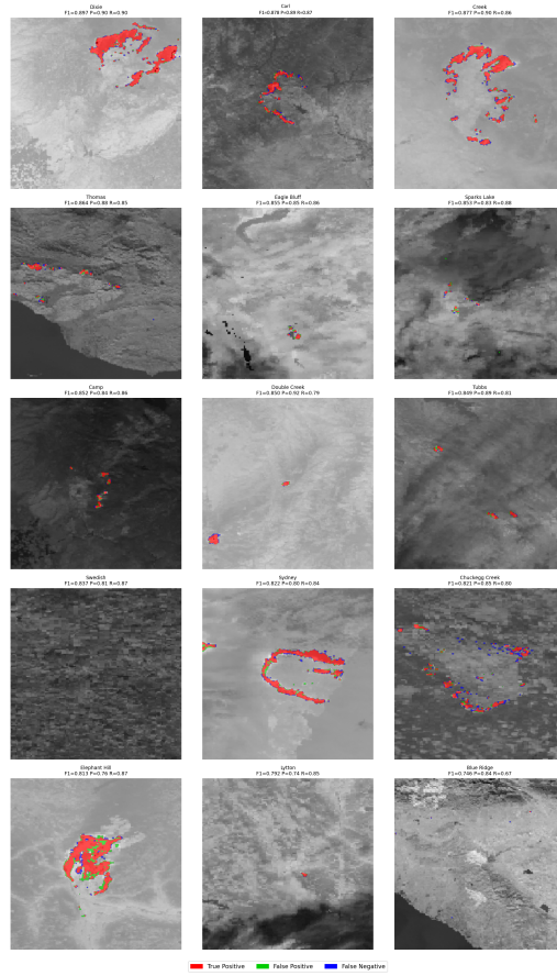
Fig. 5: AF test-set predictions (TS = 2), shown as overlays on the VIIRS day scene. Red: true positive; green: false positive; blue: false negative. Per-fire F1 reported in each panel title.
