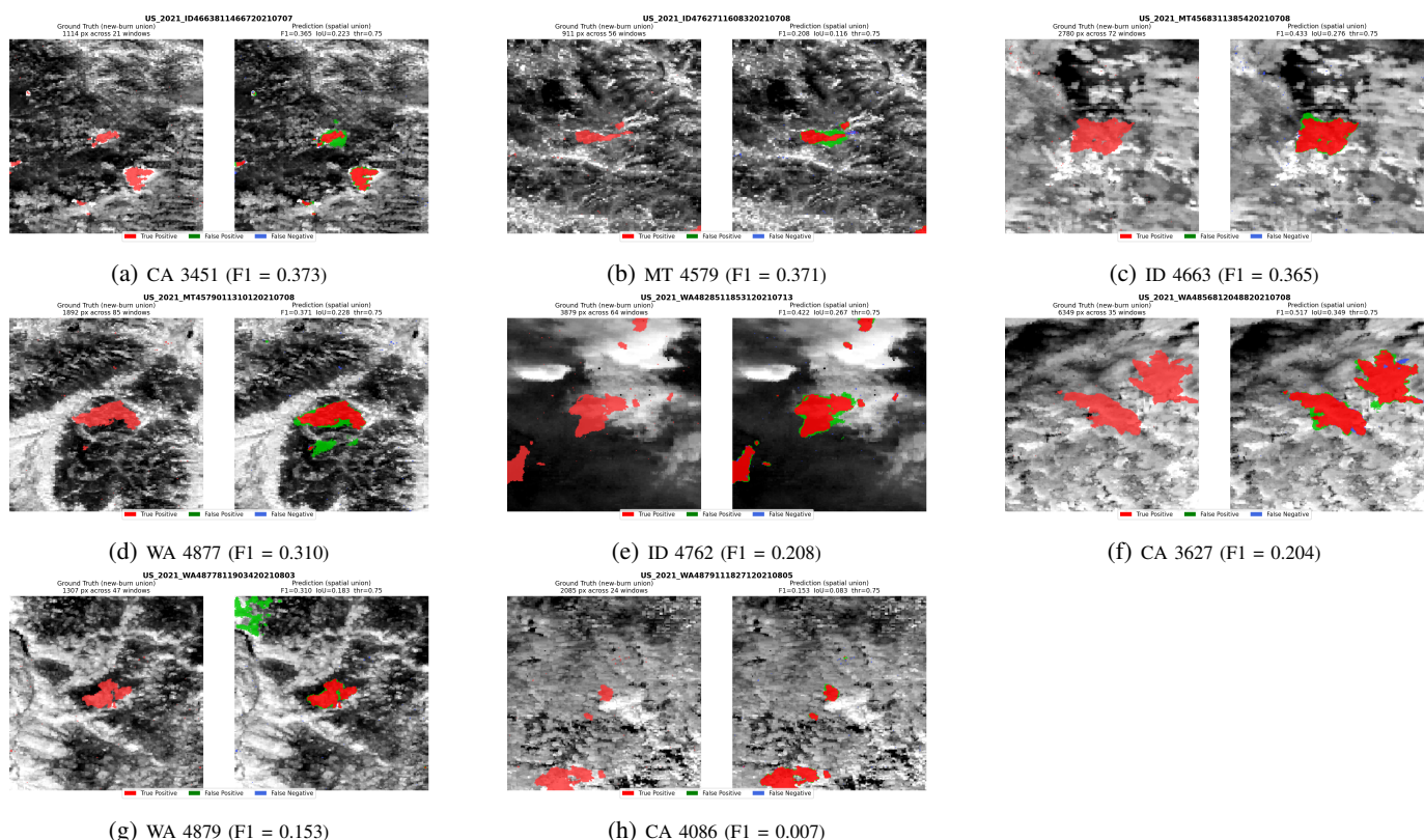
Fig. 8: Per-fire prediction maps (bottom half: 8 lower-performing US_2021 fires). Same panel layout as Fig. 7.
