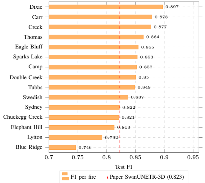
Fig. 4: Per-fire test F1 for SpaSE-UNet3D at TS = 2 on the audited AF test set (15 fires, sorted by F1). Red dashed line: SwinUNETR-3D paper baseline.
