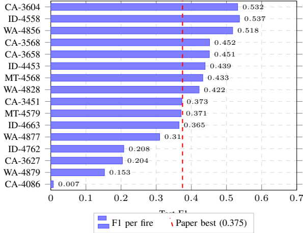
Fig. 6: Per-fire test F1 for SpaSE-UNet3D on the 16 usable US_2021 fires (sorted by F1). Six AZ/NM fires with burn fractions < 0.001% are excluded as discussed in Section IV. Red dashed line: best paper baseline (0.375).
