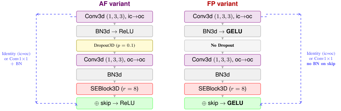
All convolutions use kernel (1, 3, 3) with padding (0, 1, 1) . The temporal dimension T is preserved through the block but never mixed across days.
