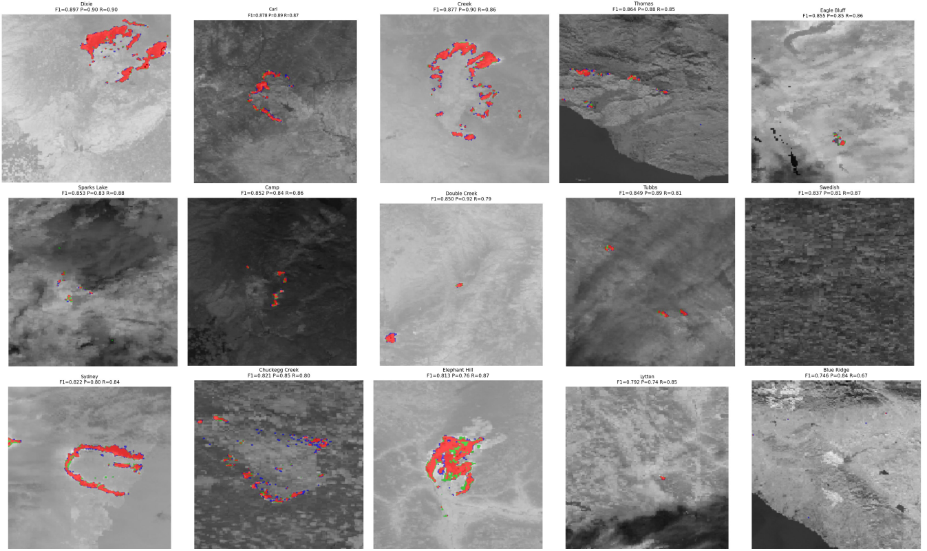
Fig. 5: AF test-set predictions (TS = 2) for the 15 audited test fires, sorted by F1 from top-left to bottom-right. Each panel overlays the per-pixel confusion mask on the VIIRS day scene: red = true positive, green = false positive, blue = false negative. Per-fire F1, precision, and recall are reported in each panel title.
