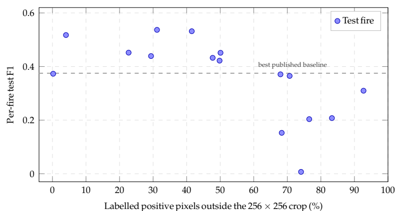
Figure 7. Per-fire fire-progression F1 against the fraction of labelled positive pixels falling outside the 256 \times 256 centre crop (Section 3.3), for the 16 fires of Fig. 8. Fires whose extent is largely cropped away score poorly regardless of model behaviour; Spearman \rho = -0.685 , p = 0.0034 , n = 16 .
