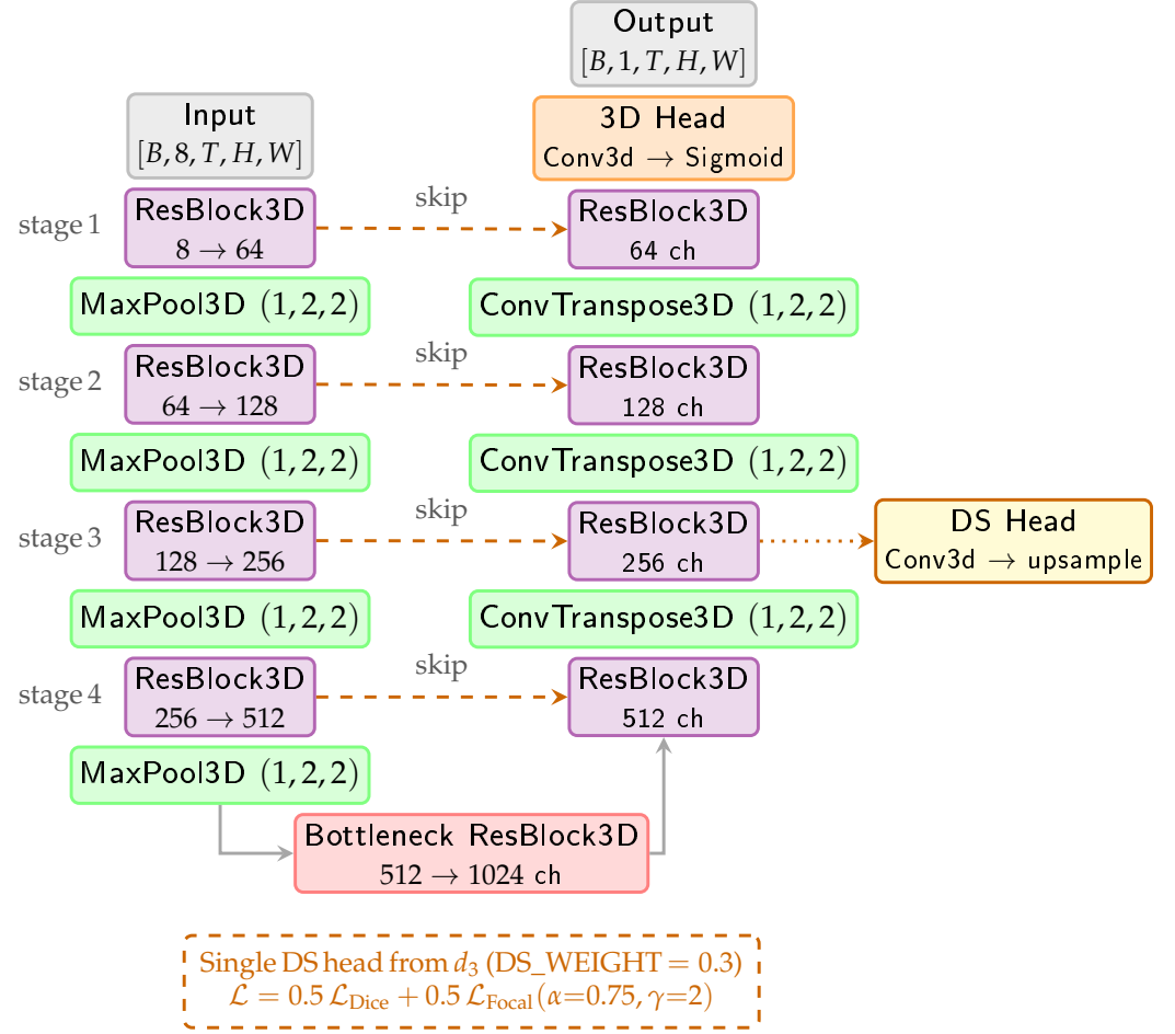
Figure 2. SpaSE-UNet3D AF variant. The encoder (left column) takes an 8-channel VIIRS input and downsamples spatially through four ResBlock3D stages with channels [64, 128, 256, 512] . A single ResBlock3D bottleneck widens to 1024 channels. The decoder (right column) mirrors the encoder with channel concatenation at every skip. A 3D head produces per-day fire masks. Deep supervision is applied at the third decoder stage.
