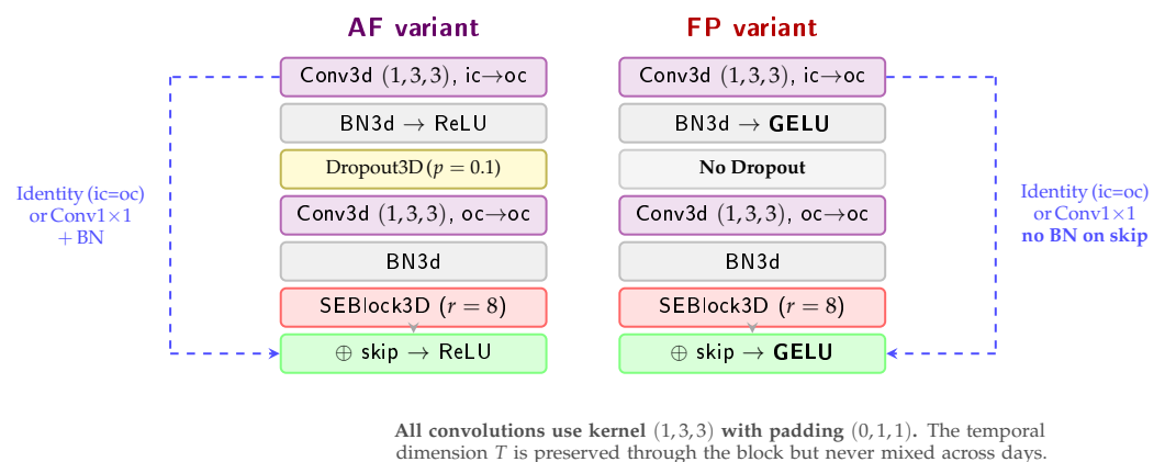
Figure 1. Internal structure of the ResBlock3D used in both SpaSE-UNet3D variants. Both blocks share spatial-only (1, 3, 3) convolutions and SE channel attention. The AF variant (left) uses ReLU activations and Dropout3D for regularisation; the FP variant (right) uses GELU and removes Dropout, which empirically hurt convergence on the smaller, sparser FP training set. The skip path either passes the input unchanged (when ic = oc ) or applies a 1 \times 1 \times 1 projection convolution.
