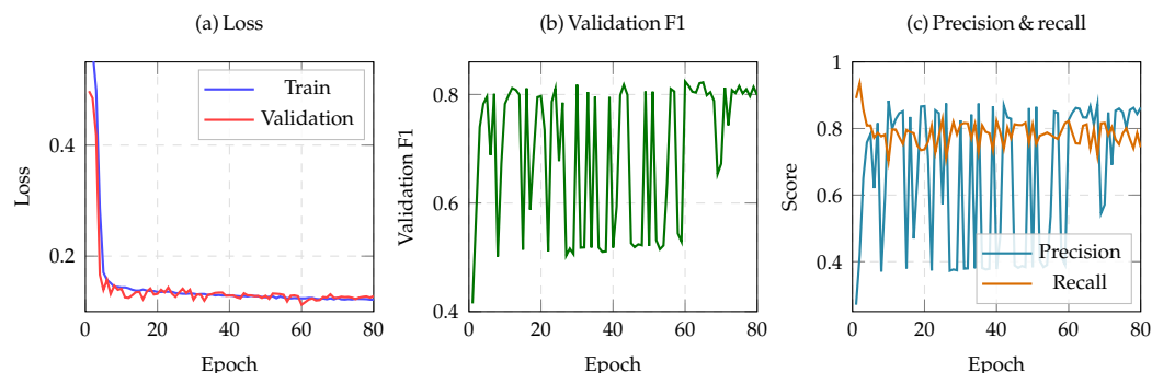
Figure 4. Training behaviour of the AF variant at TS = 2 for a representative run. (a) Training and validation loss remain closely coupled. (b) Validation F1 rises above 0.80 within ten epochs and then oscillates as the operating point moves. (c) Validation precision and recall: recall is the binding constraint for much of training, which is the behaviour the label audit of Section 4 addresses.
