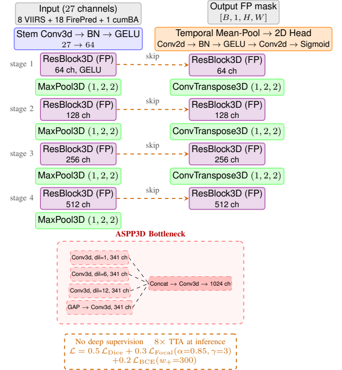
Fig. 3: SpaSE-UNet3D FP variant. The encoder takes a 27-channel input combining VIIRS, FirePred auxiliary bands, and a cumulative burned-area mask. The bottleneck is replaced with an ASPP3D module that aggregates multi-scale context via parallel dilated convolutions and a global average pool. The final head collapses the temporal dimension via a mean-pool and applies a 2D convolutional head to produce a single-day FP mask. No deep supervision is used; 8 \times test-time augmentation is applied at inference.
