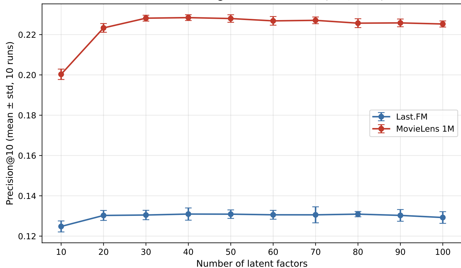
Part 3A — Precision@10 vs latent factors (BPR, k=10)
