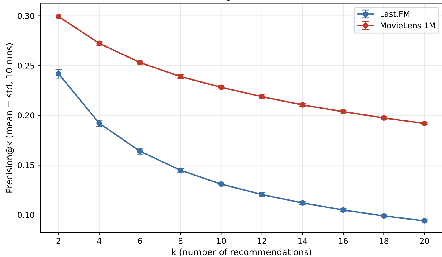
Part 3B — Precision@k vs k (BPR, factors=50)
