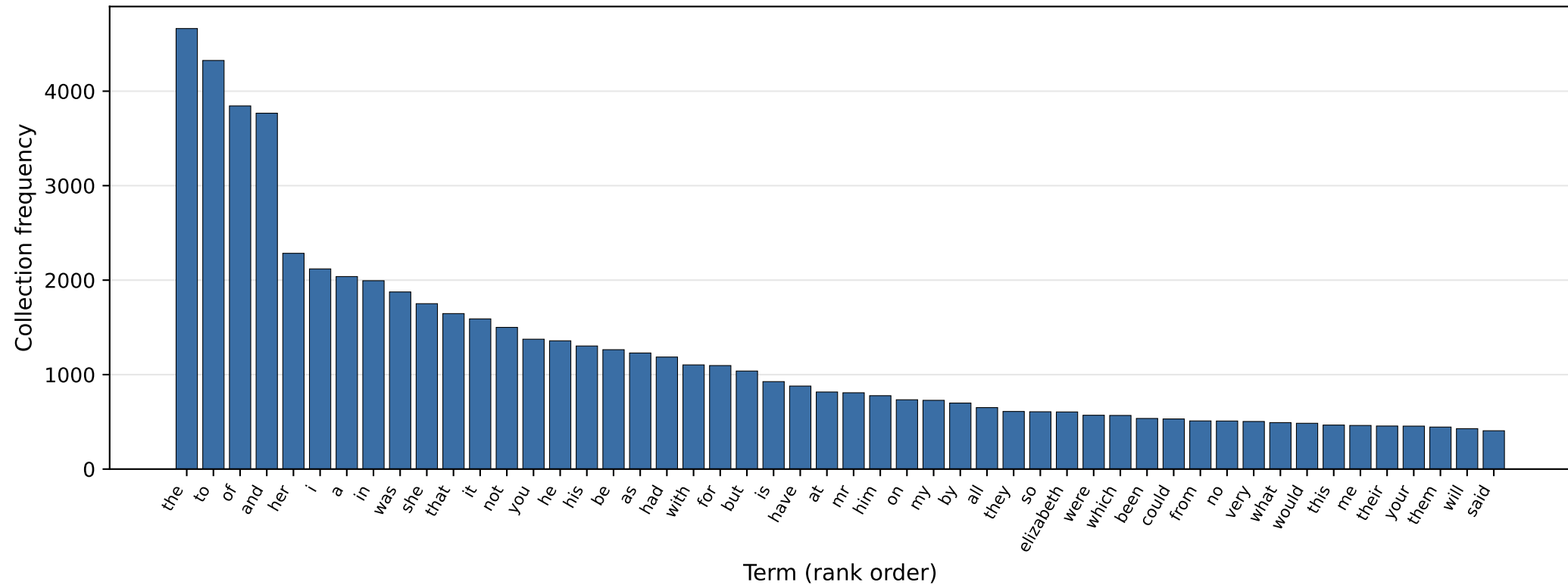
Top 50 most frequent terms in Pride and Prejudice
