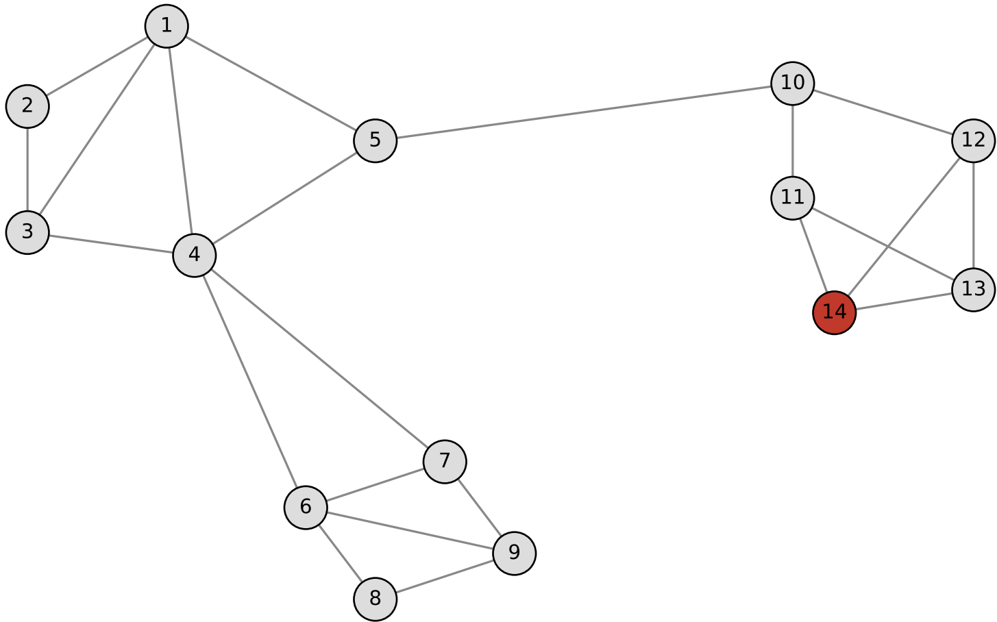
14-node undirected graph (Part 1A & 1D) Node 14 is the teleport target
