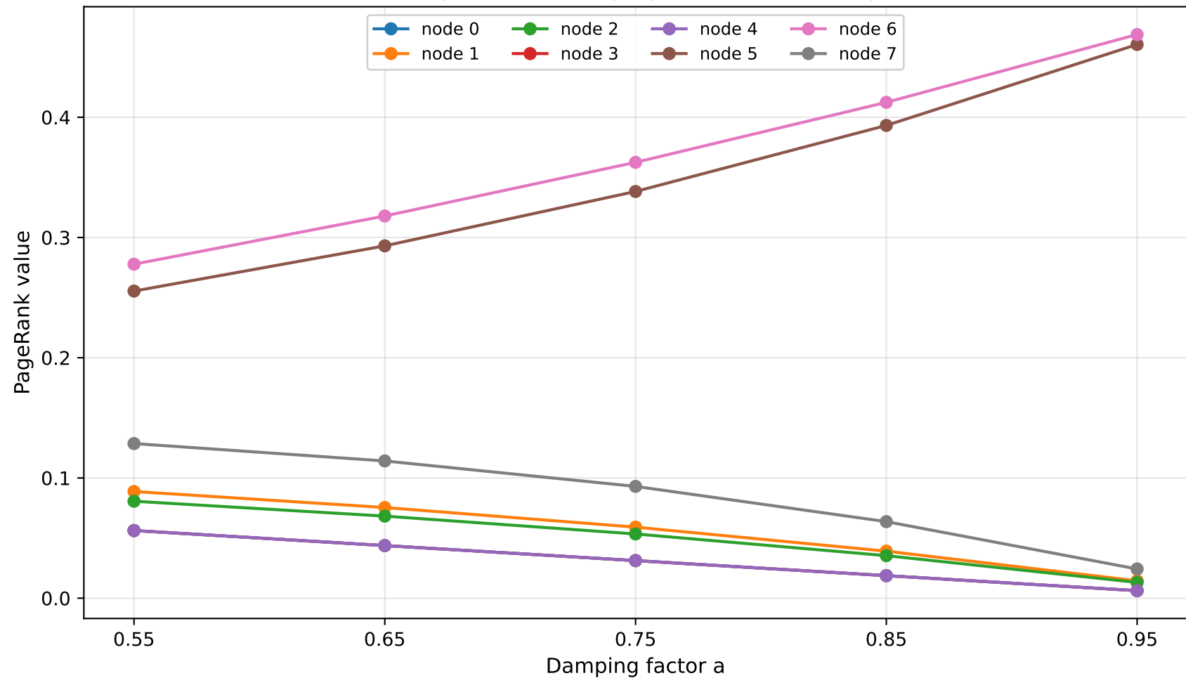
Part 1B — PageRank vs damping factor (one curve per node)
