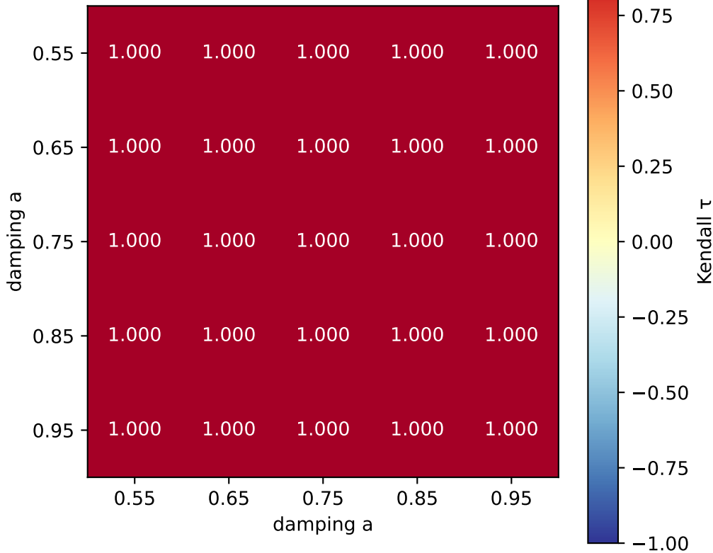
Part 1B — Pairwise Kendall \tau between rankings
