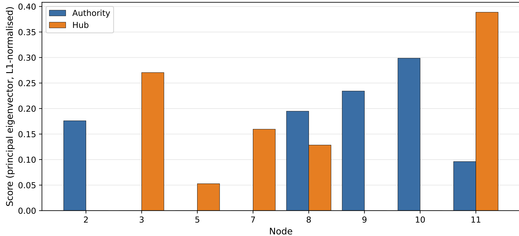
Part 1C — HITS authority and hub scores
