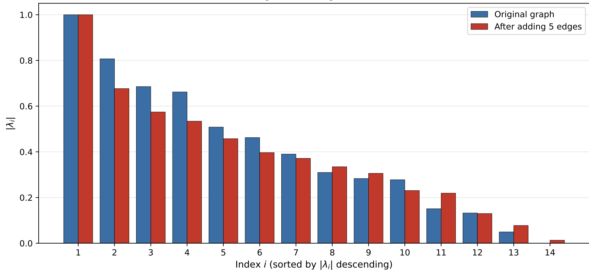
Part 1D — Google-matrix eigenvalues ( \alpha = 0.85 )
