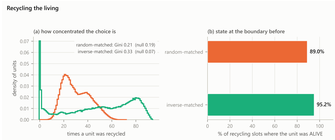
Figure 8: Which units recycling keeps choosing, and what state they were in. Per-unit recycle counts against a null that holds k fixed per task and per layer and redraws only which units, so any excess concentration is targeting rather than dose.
