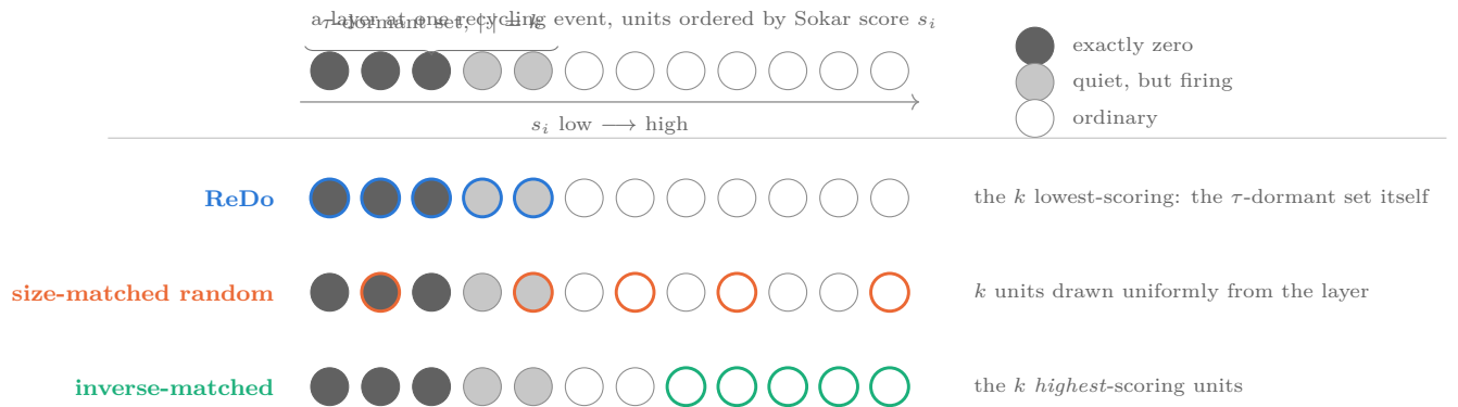
Figure 2: The three recycling arms. At every event, in every layer, the \tau -dormancy score is computed and k is set to the size of the \tau -dormant set. All three arms then recycle exactly k units by the identical procedure — re-initialise the incoming weights from the layer’s original initialisation distribution, zero the outgoing weights (Sokar et al., 2023) — and differ only in which k . Because k is recomputed per layer per event rather than fixed as a fraction or a schedule, the comparison isolates the effect of targeting from the effect of dose. Circles are units; shading is their state on the probe batch, which is measured independently of the score that selects them.
