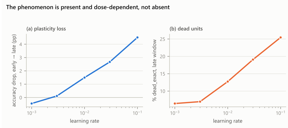
Figure 9: The gate as a dose-response in step size, both criteria. Perfect monotonicity across two decades reproduces Dohare et al.’s finding that the largest step size gives the strongest effect, as a curve rather than at a single point.
