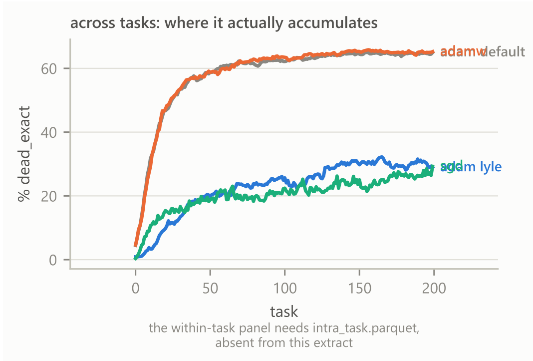
Figure 11: Where Adam’s death accumulates (Section 5.5). The panel showing the pre-registered within-task spike is not drawn : the analysis extract for these runs predates a fix to the extractor that omitted the intra-task table, and the figure states this on its face rather than shipping only the panel that worked. The intra-task numbers in Section 5.5 come from the run outputs directly.
