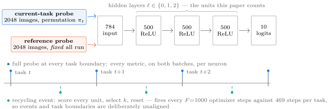
Figure 1: Setting and instrument. A 784–500–500–500–10 ReLU MLP on online permuted MNIST: each task is a fresh input permutation seen for a single pass, and the outcome measure is online accuracy, scored on the forward pass taken before each update. Every death metric is evaluated on two probe batches — the current task’s distribution and a reference distribution fixed for the entire run — and both are logged, because the gap between them is what separates a unit that is dead from one that is merely silent on the permutation being trained on right now. Per-neuron state is written at every task boundary; recycling events are governed by an optimizer-step counter rather than by task index, so they fall inside tasks rather than at their edges.
