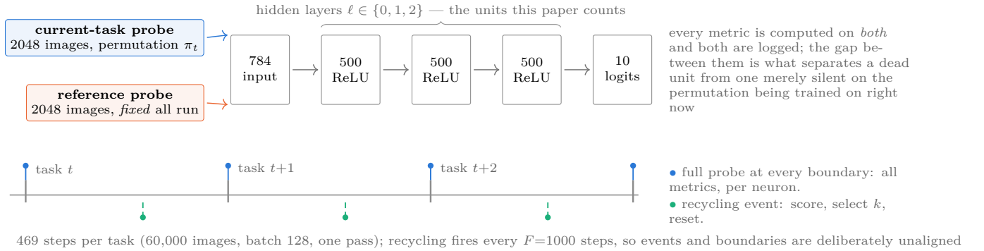
Figure 1: Setting and instrument. A 784–500–500–500–10 ReLU MLP on online permuted MNIST: each task is a fresh input permutation seen for a single pass, and the outcome measure is online accuracy, scored on the forward pass taken before each update. Every death metric is evaluated on two probe batches — the current task’s distribution and a reference distribution fixed for the entire run — and per-neuron state is written at every task boundary. Recycling events are governed by an optimizer-step counter ( F = 1000 ) rather than by task index, so they fall inside tasks rather than at their edges.
