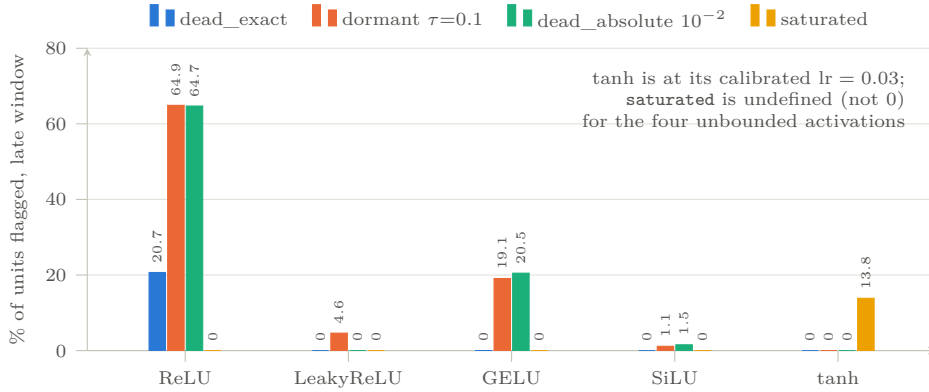
Figure 6: Four definitions across five activation functions (Table 6). The figure drops any arm within 5 pp of chance and says so on its face, so the diverged tanh-at- \text{lr}=0.1 arm cannot reach a plot by accident; the calibrated tanh arm is at \text{lr} = 0.03 .
