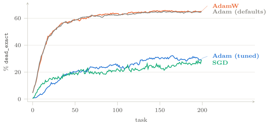
Figure 11: Where Adam’s death accumulates : across tasks, not within them. Adam and AdamW track each other almost exactly, which is the point of including both. The panel showing the pre-registered within-task spike is not drawn — the analysis extract for these runs predates a fix to the extractor that omitted the intra-task table, and the figure states this on its face rather than shipping only the panel that worked. The intra-task numbers below come from the run outputs directly.
