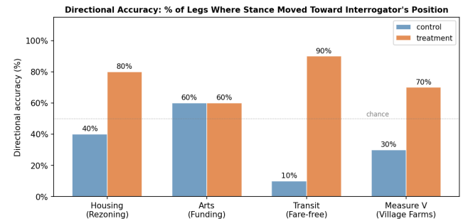
Figure 1: Directional accuracy (%) by topic and condition. The dashed line at 50% marks direction-agnostic drift. Treatment exceeds control on 3 of 4 topics.
