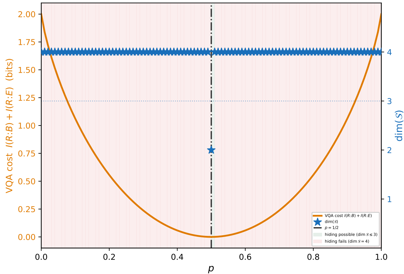
Bell Mixture State \rho(p) = p |\Phi^+\rangle\langle\Phi^+| + (1-p) |\Psi^+\rangle\langle\Psi^+|
