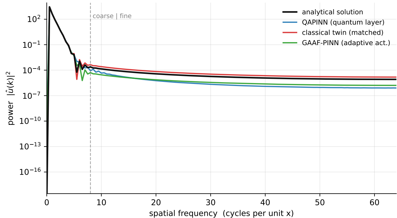
Output Fourier spectrum - burgers n4, t = 1.00 (seed 1234)
