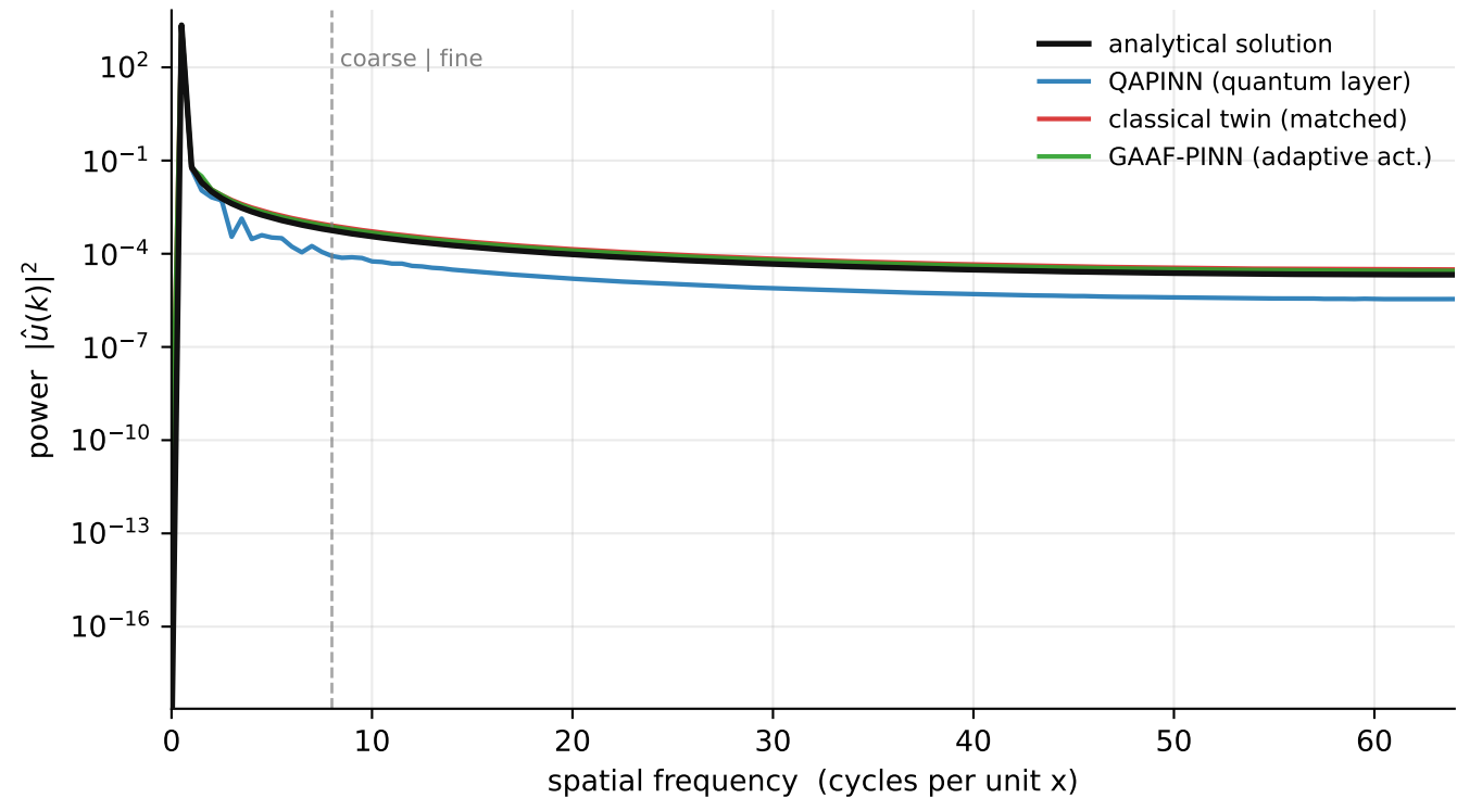
Output Fourier spectrum - heat n6, t = 1.00 (seed 1234)
