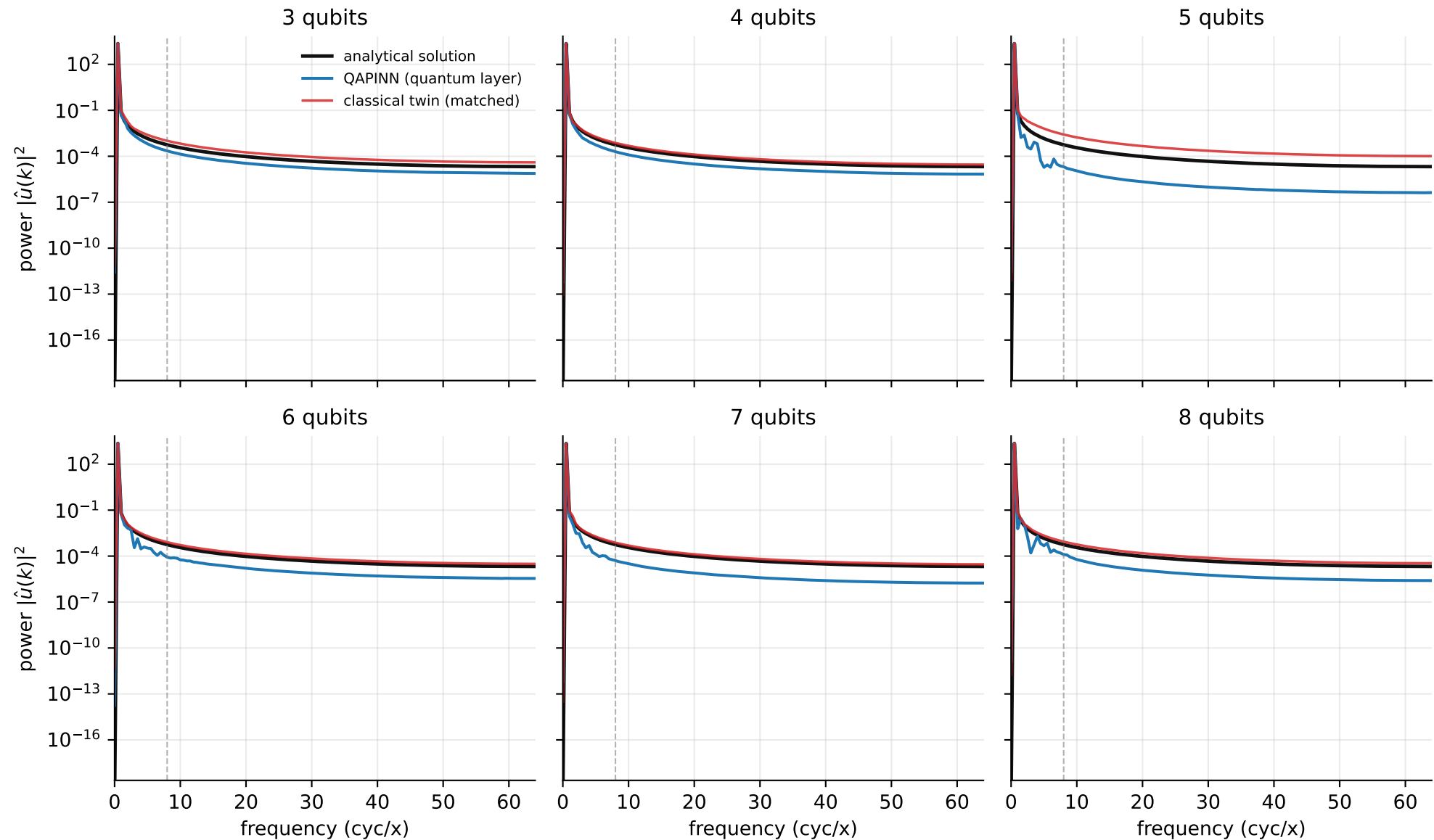
Output Fourier spectrum vs qubit count - heat (t=1.00, seed 1234)
