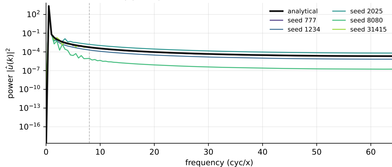
qapinn spectrum, all seeds - heat n4 (t=1.00)
