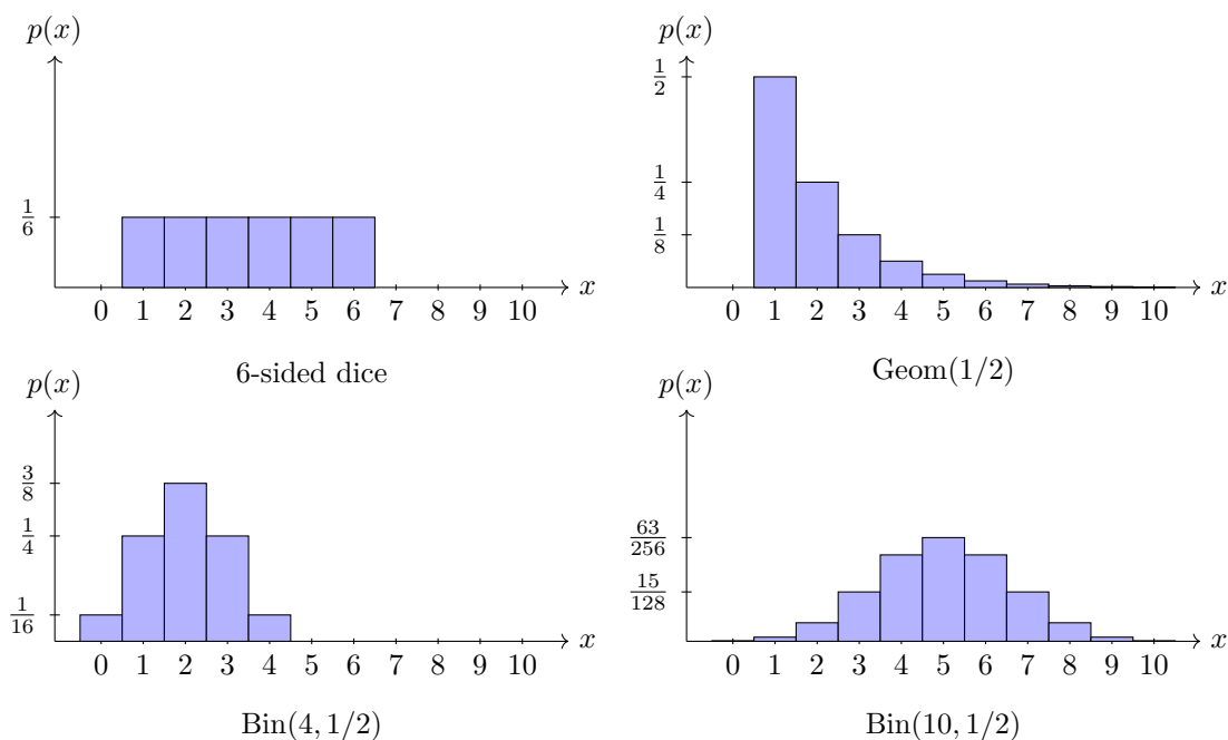
Figure 1: The distributions for a 6-sided dice (top left), the coin-flipping random variable from Example 4 (top right), and binomial random variables with parameters (n, p) = (4, .5) (bottom left) and (n, p) = (10, .5) (bottom right).
