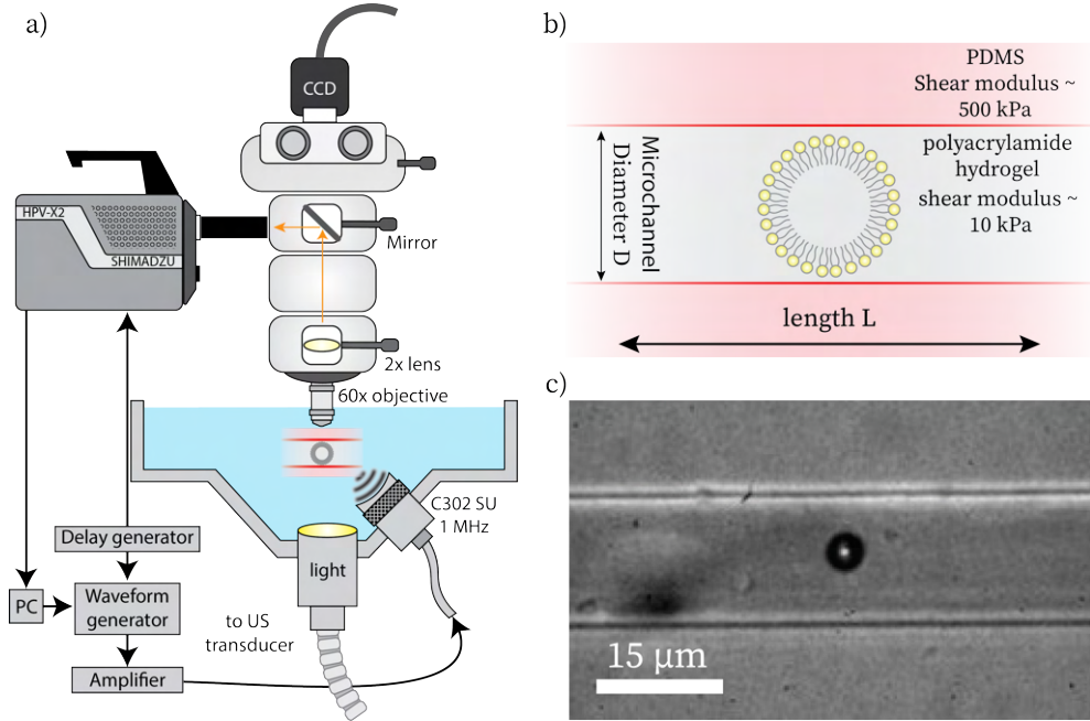
Figure 5.1: a) Optical characterization setup b) Schematic of a PDMS microchannel containing a phospholipid-coated microbubble c) Microscopy image of a bubble in a microchannel of diameter D = 15 \mu\text{m} .
