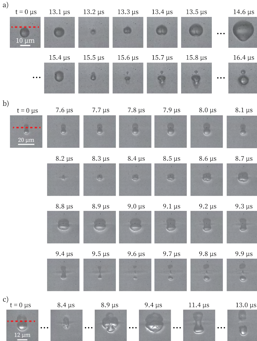
Figure 6.2: a) A bubble floating against a polyacrylamide hydrogel with a shear modulus of 70 kPa, driven by an 8-cycle pulse at 300 kPa pressure at a frequency of 1.0 MHz. b) A bubble floating against a polyacrylamide hydrogel with a shear modulus of 200 kPa, driven by a 1-cycle pulse at 500 kPa pressure and a frequency of 1.0 MHz. Note the surface deformation and the traveling wave in the hydrogel. c) Visible surface damage to a polyacrylamide hydrogel with a shear modulus of 200 kPa at t = 13.0 \mu\text{s} , driven by a 1-cycle pulse at 500 kPa pressure and a frequency of 1.0 MHz.
