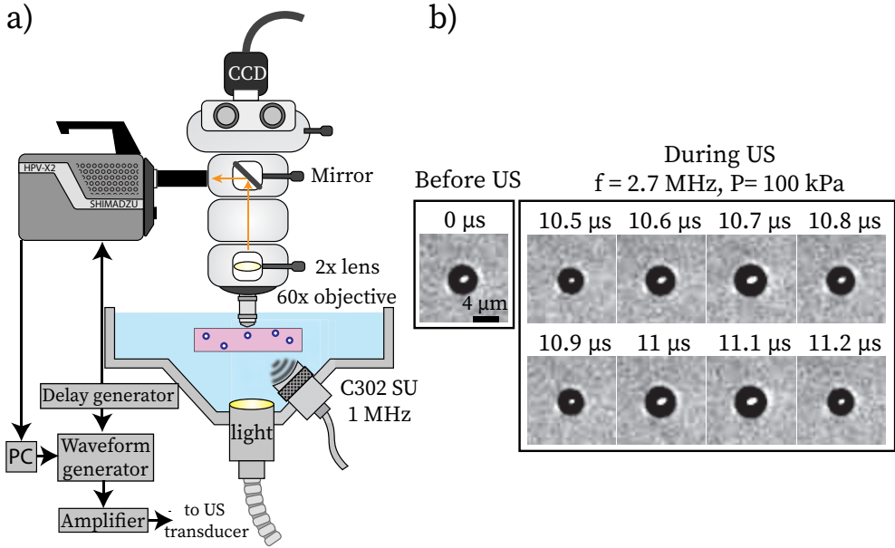
Figure 2.2: (a) Schematic of the experimental setup. (b) Snapshots of an ultra-high-speed recording of an oscillating microbubble with an initial radius of R_0 = 1.7 \mu m in a soft hydrogel with a shear modulus of G(\omega \rightarrow 0) \approx 70 kPa. The interframe time is 100 ns.
