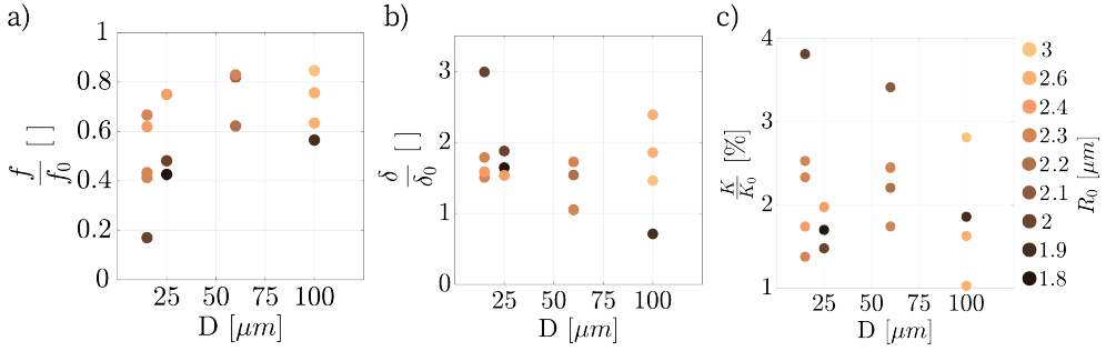
Figure 5.3: a) Ratio of the resonance frequency of the bubble in the tube to that of the same bubble in free field, plotted against the diameter of the microchannel. b) Damping coefficient in the microchannel normalized by the damping in an unconstrained medium as a function of the diameter of the microchannel. c) Ratio between the gain in the microchannel and the free-field gain versus the microchannel diameter.
