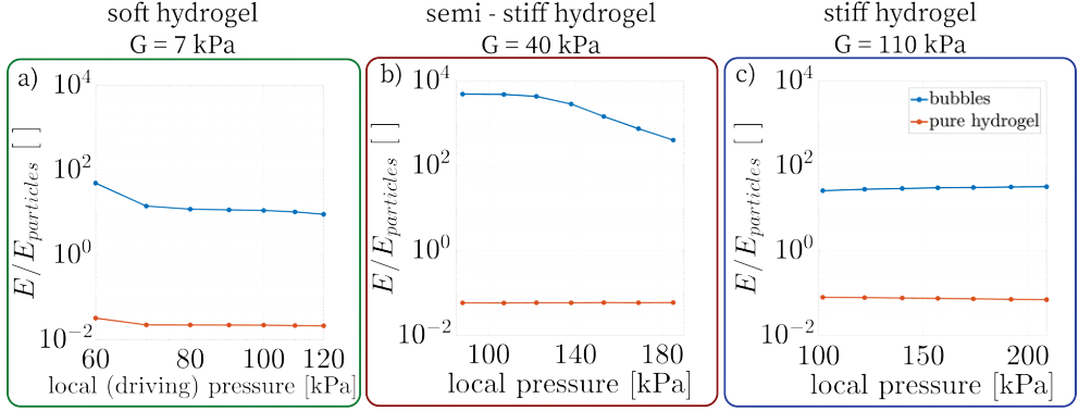
Figure 4.5: Scattered energy from the pure and bubble-containing hydrogels relative to the energy scattered from the particle-containing hydrogels for the a) soft, b) semi-stiff, and c) stiff hydrogels.
