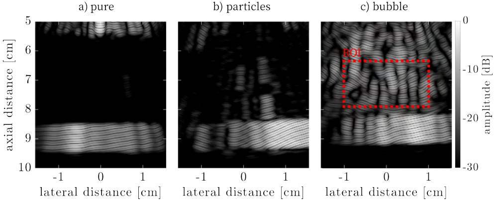
Figure 4.3: Reconstructed images in a semi-stiff hydrogel a) pure, b) loaded with particles, and c) loaded with bubbles. The images were acquired at an acoustic pressure of 60 kPa and a frequency of 2.0 MHz. In all images, the reflection of pressure waves from the back wall of the samples is visible at an axial distance of 9 cm.
