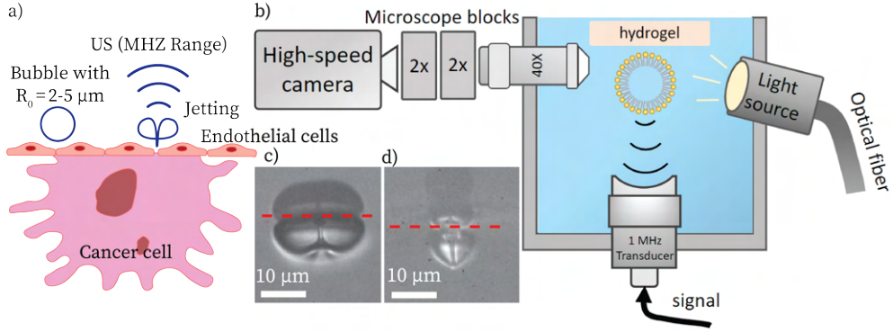
Figure 6.1: a) Schematic of a liquid jet penetrating the endothelial wall of a vessel and interacting with a cancer cell. b) Side-view setup for capturing liquid jets. c) Liquid jet directed toward a solid microscope slide with a thickness of 1 mm, driven by a 500 kPa pressure, 1 cycle, and 1 MHz frequency. d) Liquid jet moving outward from the surface of a gel with a shear modulus of 200 kPa, driven by 500 kPa pressure, 8 cycles, and 1 MHz frequency.
