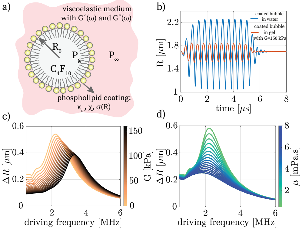
Figure 2.1: (a) Schematic and relevant parameters for a phospholipid-coated microbubble in a viscoelastic medium. (b) Radial response for a coated bubble in water ( \mu = 1 mPa.s) and in a viscoelastic medium ( G = 150 kPa and \mu = 1 mPa.s). (c) Resonance curves of a coated microbubble in media with a viscosity of \mu = 1 mPa.s and G ranging from 0 to 150 kPa. (d) Resonance curves of a coated microbubble for media with G = 0 Pa and \mu ranging from 1 to 8 mPa.s.
