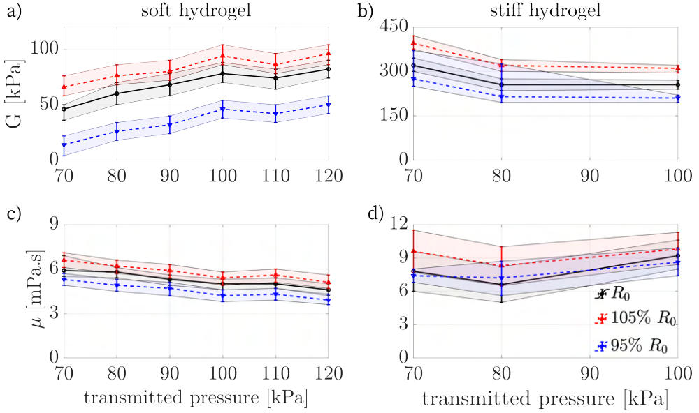
Figure 2.4: (a) and (b) Extracted values of G for the soft and stiff hydrogels, respectively, using RMSE minimization. (c) and (d), viscosity as a function of the driving pressure for both hydrogels. The error bars (and shadowed region) represent the results for the same bubble but for \pm 10\% of the acoustic pressure to assess the effect of calibration uncertainties. Due to the sizing error of microbubble G and \mu are also calculated for radii with \pm 5\% change. These are shown by the red and blue dashed lines.
