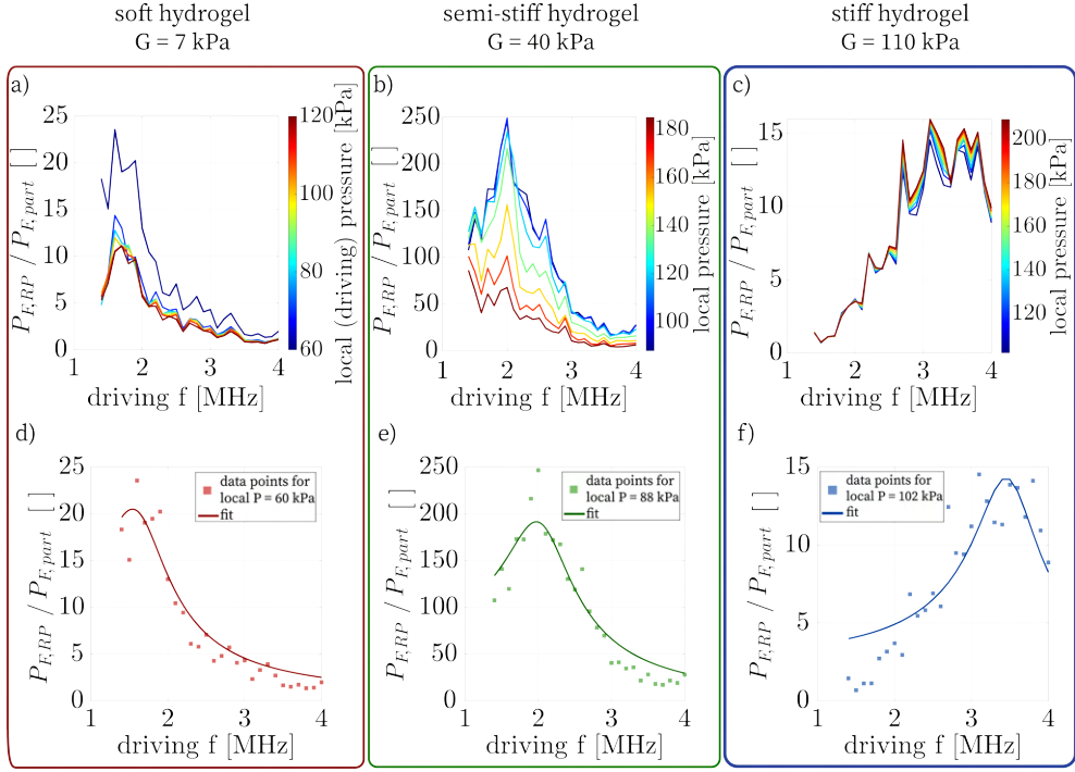
Figure 4.4: a, b, c) Resonance curves of bubbles in soft, semi-stiff, and stiff hydrogels, respectively, for various acoustic pressures. d, e, f) Fit of the resonance curves acquired with the lowest local pressure, i.e., 60, 88, and 102 kPa in the soft, semi-stiff, and stiff hydrogels.
