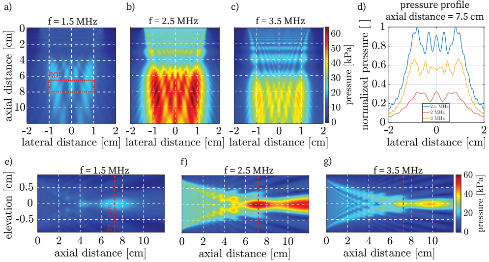
Figure 4.2: Simulated pressure fields in the axial-lateral plane at a) 1.5 MHz, b) 2.5 MHz, and c) 3.5 MHz. d) Pressure profile at a fixed distance of 7.5 cm from the surface of the transducer, corresponding to the middle of the sample normalized to the maximum pressure. e, f, g) Pressure fields for elevational-axial plane. The elevation axis is increased by a factor 3 for a better visualization.
