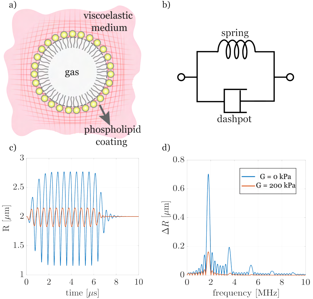
Figure 1.1: a) Schematic of a phospholipid-coated microbubble in a viscoelastic medium. Upon exposure to ultrasound, the bubble deforms the material. b) Schematic of the linear Kelvin-Voigt model. Elastic (spring) and viscous (dashpot) components are in a parallel configuration. c) Radius vs. time curves for the bubble with R_0 = 2.0 \mu\text{m} . The blue curve is for a coated microbubble with \sigma(R_0) = 20 \text{ mN/m} that is driven at its resonance frequency ( f_0 = 1.8 \text{ MHz} ) by P_{ac} = 100 \text{ kPa} in water G = 0 \text{ kPa} . d) Frequency spectra of the graphs in panel c.
