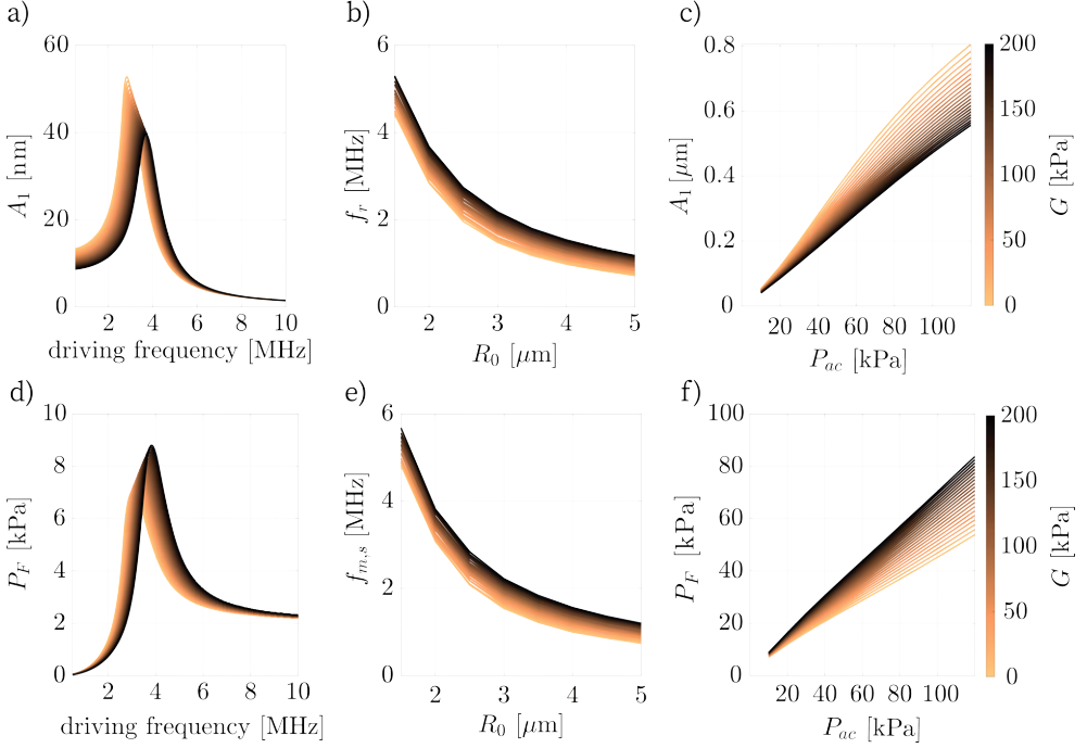
Figure 3.2: a) Amplitude of oscillation at the fundamental frequency A_1 as a function of driving frequency for R_0 = 2.0 \mu\text{m} and P_{ac} = 10 \text{ kPa} . b) Resonance frequency f_r as a function of R_0 for varying elastic moduli G and P_{ac} = 10 \text{ kPa} . c) Fundamental oscillation amplitude A_1 of R(t) versus driving pressure P_{ac} . d) Fundamental scattered pressure amplitude P_F as a function of the driving frequency for R_0 = 2.0 \mu\text{m} and P_{ac} = 10 \text{ kPa} . e) Frequency of maximum scatter as a function of R_0 for P_{ac} = 10 \text{ kPa} and for varying elastic moduli G . f) Maximum scattered pressure as a function of driving pressure P_{ac} for various elastic moduli.
