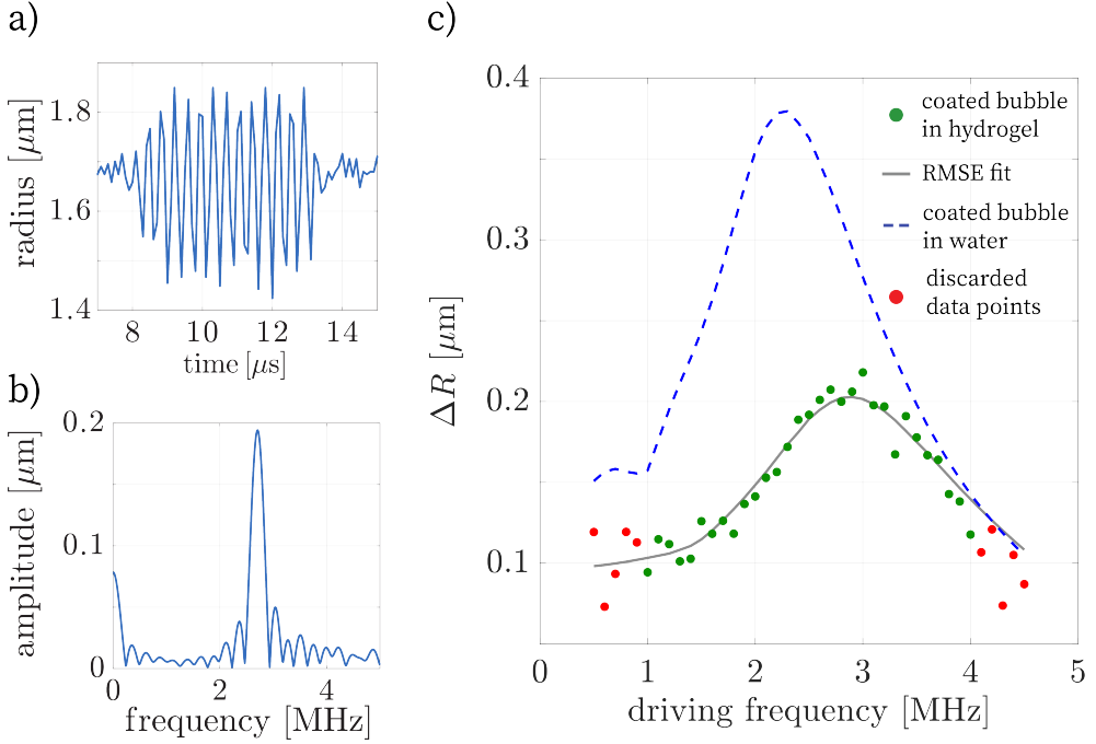
Figure 2.3: (a) Bubble radius versus time curve, extracted from a high-speed recording. The bubble was driven at a frequency of 2.7 MHz and at a pressure of 100 kPa. Panel (b) shows the Fast Fourier Transform of the data presented in (a). In (c), the resonance curve obtained from 41 high-speed recordings is shown with a best fit to the experimental data obtained through RMSE minimization. In this figure, the best-fit parameters were G \approx 70 kPa, \mu = 5.6 mPa.s, and P_{ac} = 100 kPa. The blue dotted line represents the simulated resonance curve for the very same bubble in water.
