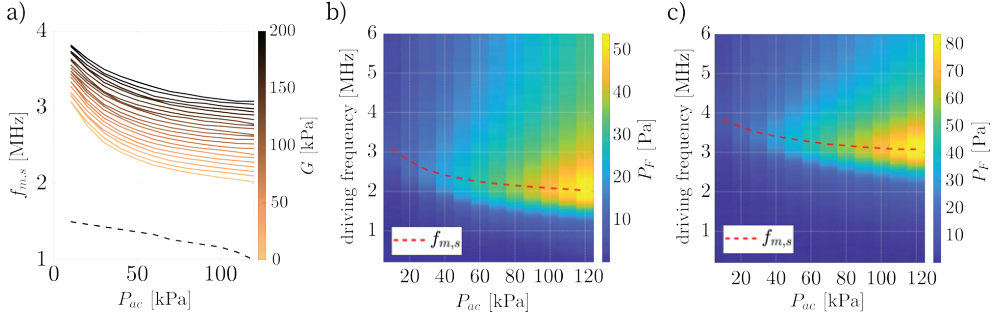
Figure 3.3: Interplay between phospholipid shell and viscoelastic medium for a bubble with R_0 = 2.0 \mu\text{m} . a) Resonance frequency as a function of driving pressure. The dashed black line corresponds to the resonance frequency of an uncoated bubble in free field. b) and c) 2D maps describing the amplitude of the scattered pressure as a function of driving frequency and driving pressure for G = 0 \text{ kPa} and G = 200 \text{ kPa} , respectively.
