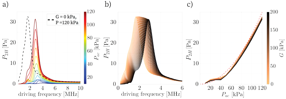
Figure 3.4: a) Maximum scattered pressure at the second harmonic for a bubble with R_0 = 2.0 \mu\text{m} as a function of driving frequency for different pressures in a medium with G = 200 kPa. The dashed line represents the resonance frequency of the same bubble in water at P_{ac} = 120 kPa. b) Maximum amplitude of the second harmonic for a bubble with R_0 = 2.0 \mu\text{m} in media with different elastic moduli (driven at P_{ac} = 120 kPa). c) Maximum amplitude of the second harmonic as a function of driving pressure for a R_0 = 2.0 \mu\text{m} bubble. The red dashed line is a guide to the eye showing a quadratic relation of the second harmonic scatter to the acoustic driving pressure
