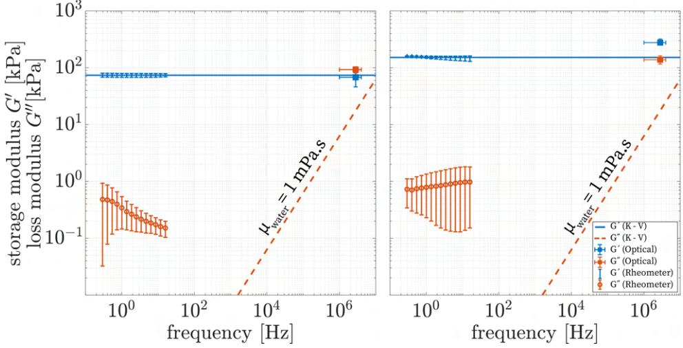
Figure 2.5: A comparison between the data obtained at low strain rates ( <16 \text{ s}^{-1} ) using a rotational rheometer and at high strain rates ( >10^6 \text{ s}^{-1} ) using ultra-high-speed imaging of the microbubble oscillations. The horizontal error bars of optical measurements suggest that the G' and G'' are measured across a range of frequencies by utilizing the resonance curves of the microbubbles. The vertical error bars originate from the standard deviation between all the measurements.
