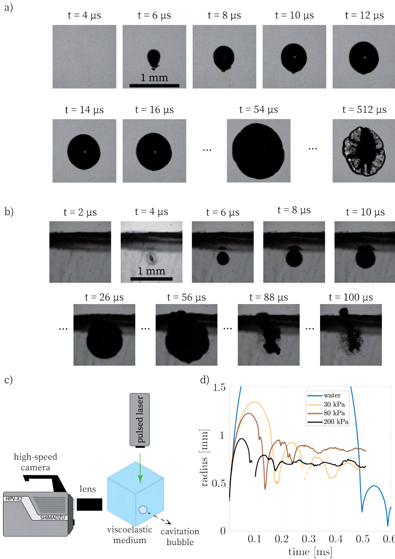
Figure 6.4: Laser-generated cavitation bubbles were created using a pulsed Nd:YAG laser with an 8 ns pulse width inside a polyacrylamide hydrogel with an elastic modulus of 200 kPa. The dynamics were recorded using a high-speed camera operating at 0.5 million frames per second. a) Bubble dynamics inside the hydrogel, far from boundaries. b) Bubble dynamics near the boundary with water. c) Schematic of the experimental setup. d) Radius-time curve extracted from the high-speed recordings.
