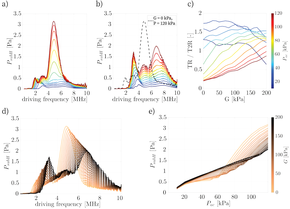
Figure 3.5: Maximum amplitude of the subharmonic for a bubble with R_0 = 2.0 \mu\text{m} as a function of driving frequency in media with a) G = 0 kPa and b) G = 200 kPa. c) Ratio of the TR to T2R subharmonic amplitudes. d) Amplitude of the subharmonic response as a function of the frequency in media with elastic moduli ranging from 0 to 200 kPa, for a bubble with R_0 = 2.0 \mu\text{m} driven at 120 kPa. e) Maximum amplitude of P_{subH} as a function of driving pressure.
