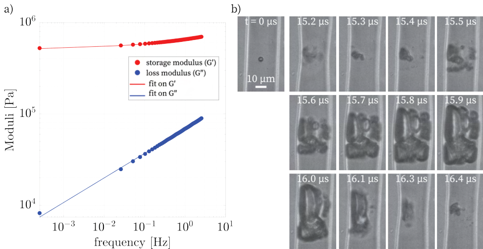
Figure 5.6: a) Rheometer frequency sweep measurement of PDMS with a shear strain of 0.1 %. The data points are fitted with a Chasset-Thirion model b) Frames from an ultra-high-speed recording. A R_0 = 2.2 \mu m bubble in a D = 25 \mu m channel, driven with an acoustic wave with f = 1 MHz, P_{ac} = 3 MPa, and a duration of 10 cycles.
