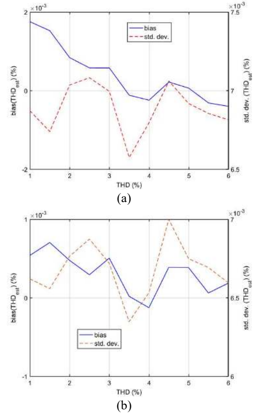
Fig. 2. Bias and standard deviation of the THD measurements achieved by the EB algorithm (a) and the two-point IpDFT algorithm (b) versus THD when the waveform frequency is f = 49.5 Hz. Analyzed waveforms affected by the first 15 harmonics and wideband noise of SNR = 50 dB. For each THD 1000 runs of M = 4096 samples each with random phases of all signal tones.
