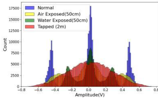
Fig. 6. Amplitude Histogram for 100BASE-TX signals acquired by the oscilloscope.
