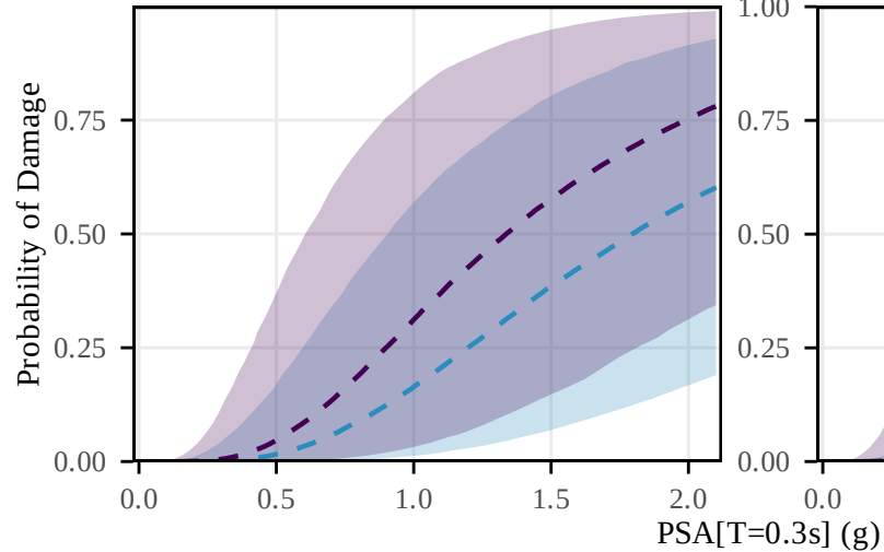
RC Wall (1-3 Storeys)
