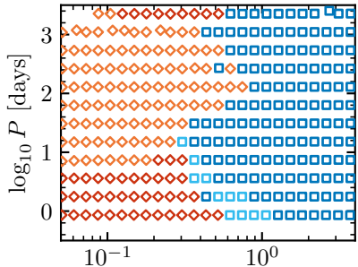
Eddington-limited
