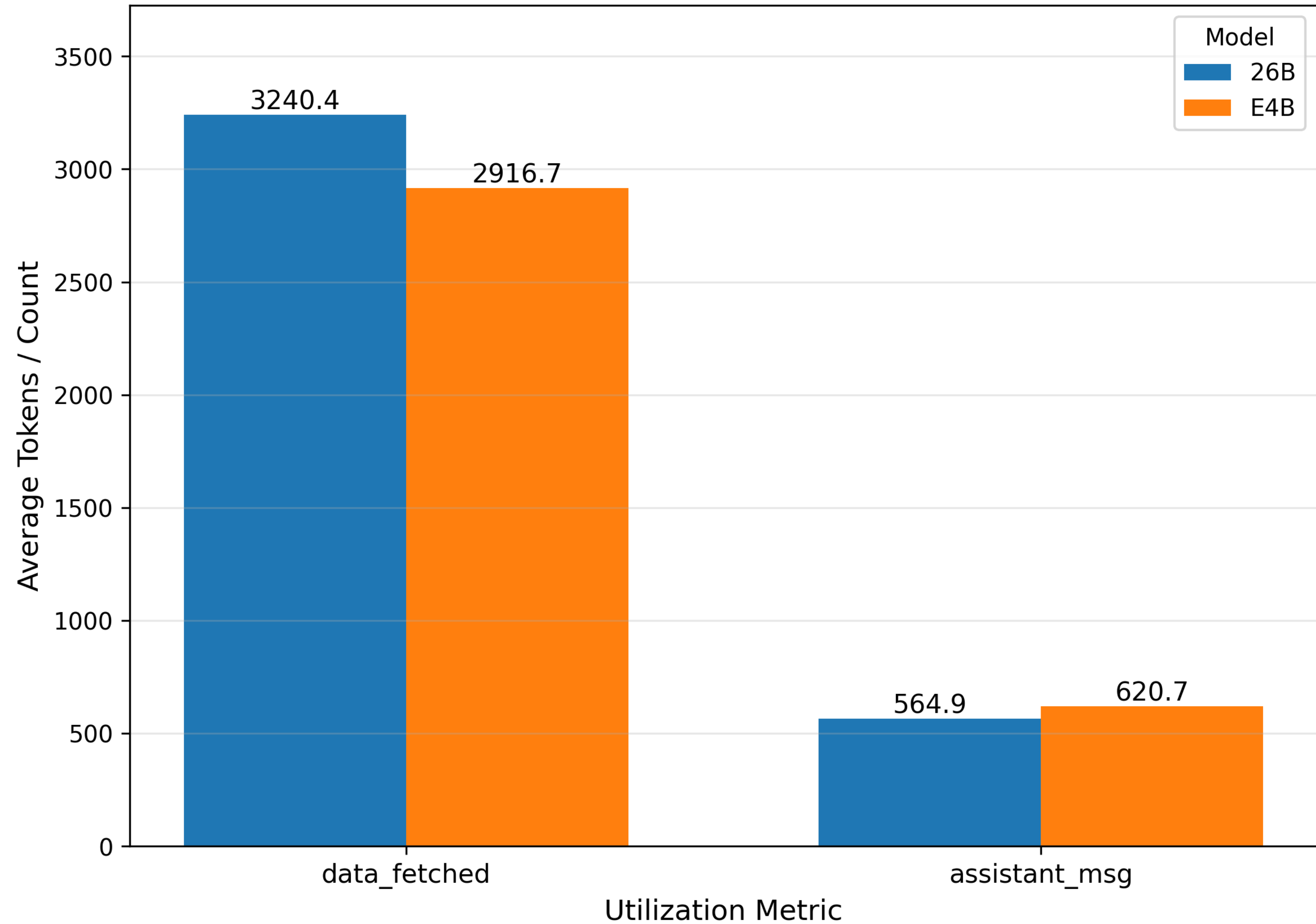
Average Context Utilization (Data vs. Assistant)
