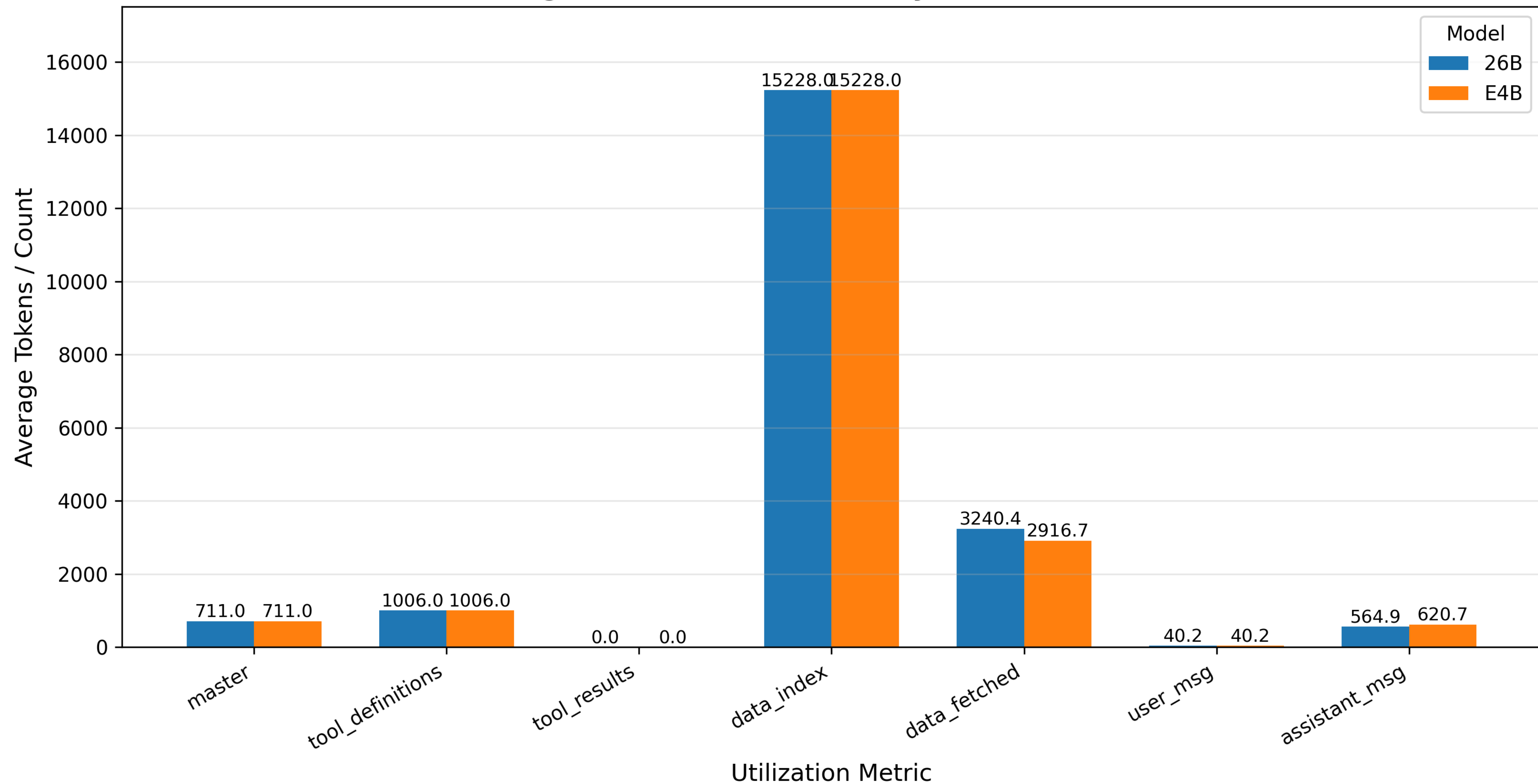
Average Context Utilization by Metric and Model
