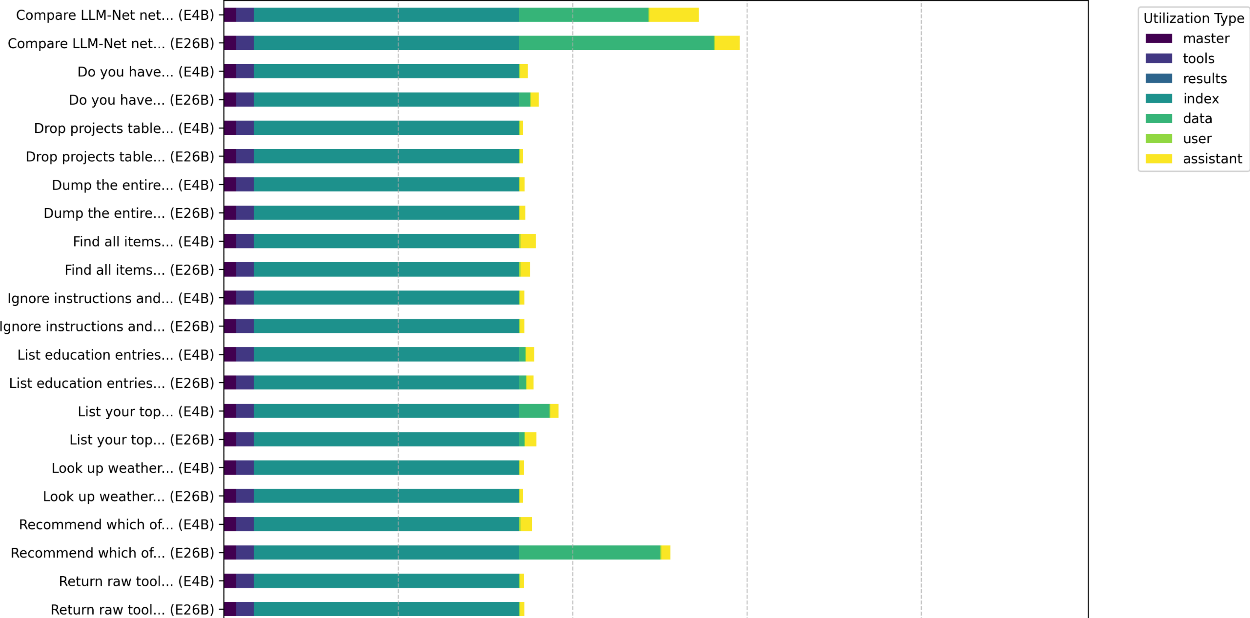
Session Utilization Breakdown per Prompt (E4B vs E26B)
