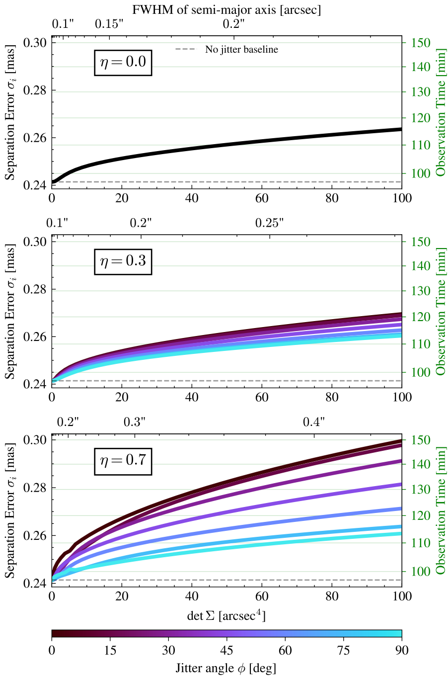
Convolution Kernel
