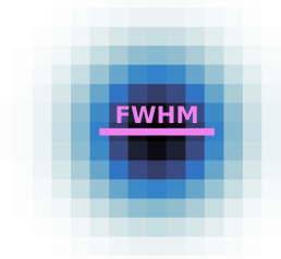
Convolution Kernel
