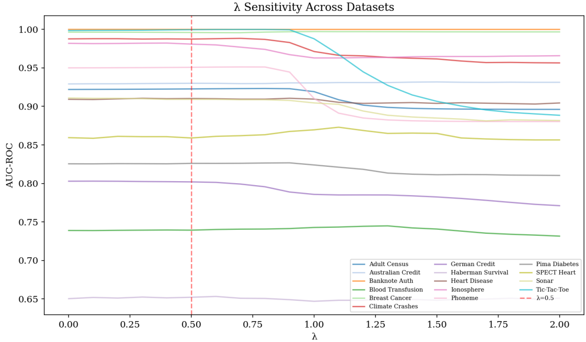
Figure 4.7: AUC-ROC as a function of \lambda for all 15 datasets. The red dashed line marks the proposed default \lambda = 0.5 . Easy datasets (top, near 1.0) are flat, as \lambda does not matter when all models are already excellent. Moderate datasets (middle) peak around \lambda = 0.5 – 0.8 . Difficult datasets (bottom) are more variable and often prefer larger \lambda . The non-parallel curves confirm that the optimal \lambda is dataset-dependent, ruling out a universal fixed default.
