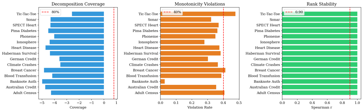
Figure 4.4: Three diagnostic checks across all 15 datasets (averaged over 5 seeds). Left: Decomposition coverage is universally negative because pairwise redundancy terms outweigh singleton contributions; the 80% threshold (red dashed line) is never met. Center: Monotonicity violation rates mostly fall between 20% and 45%, indicating that adding a model sometimes reduces coalition performance. Right: Rank stability (Spearman r ) is uniformly 1.0 across all runs and seeds.
