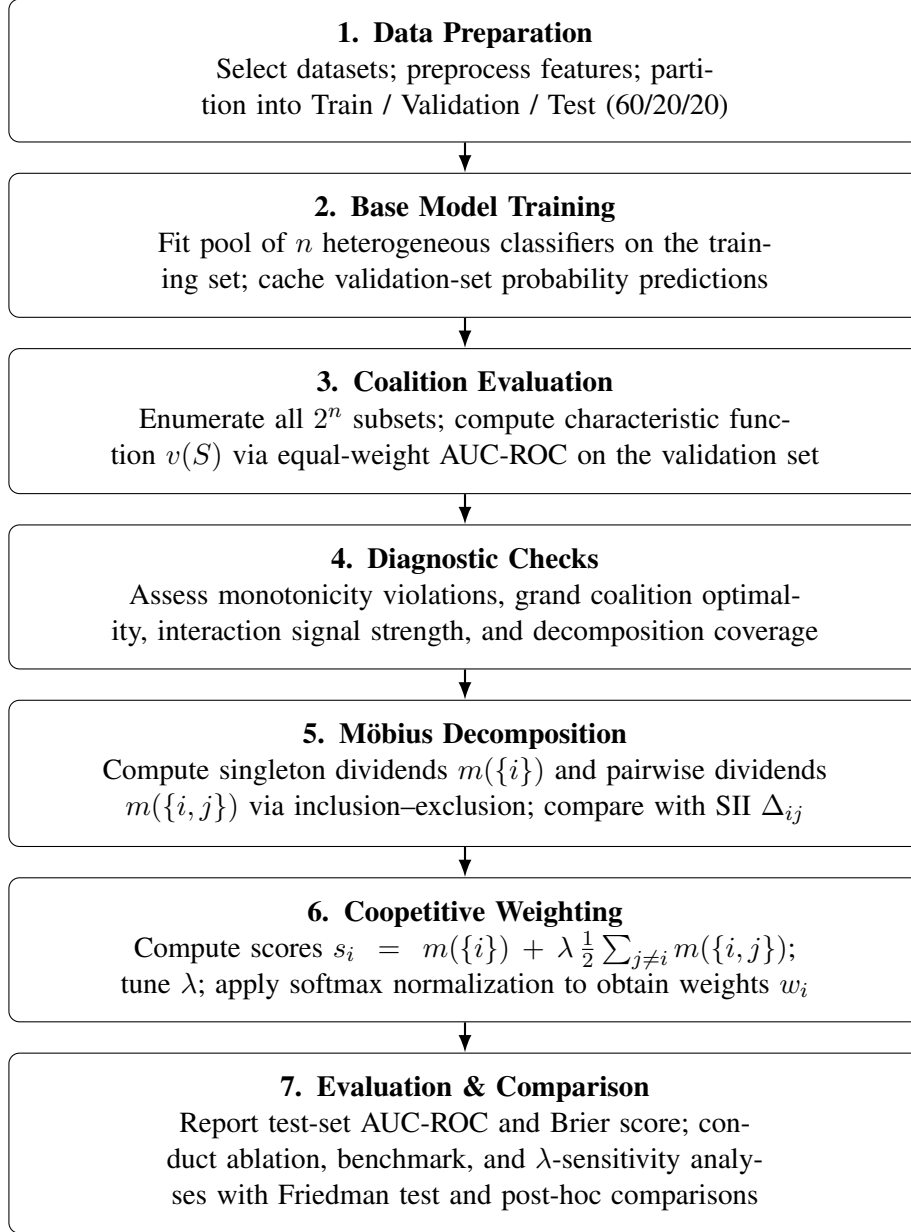
Figure 3.1: End-to-end flow of the Coopetitive Ensembling Framework evaluation, organized by logical phase.
