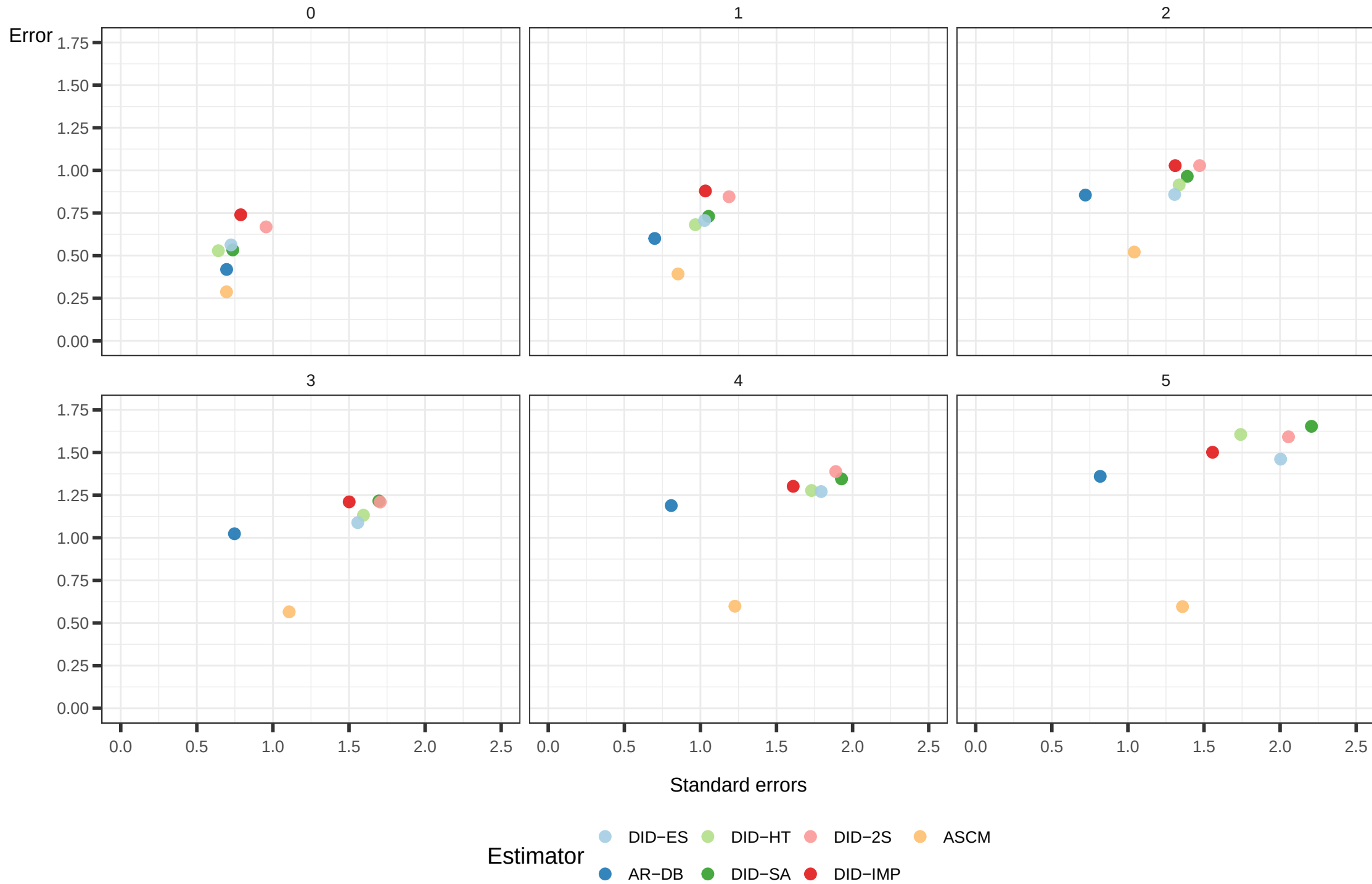
Median absolute error and standard errors by time-since-treatment: Ramp Down scenario
