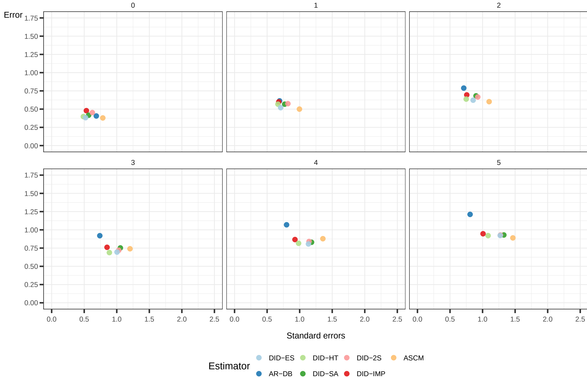
Median absolute error and standard errors by time-since-treatment: Ramp Up scenario
