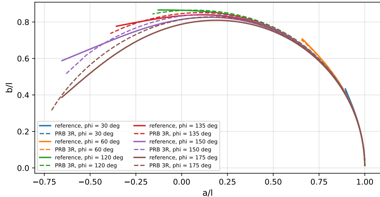
PRB 3R Force Angle Sweep
