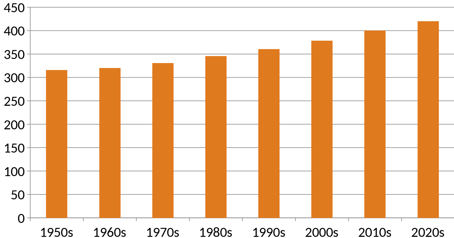
Mean CO2 by decade (ppm)
