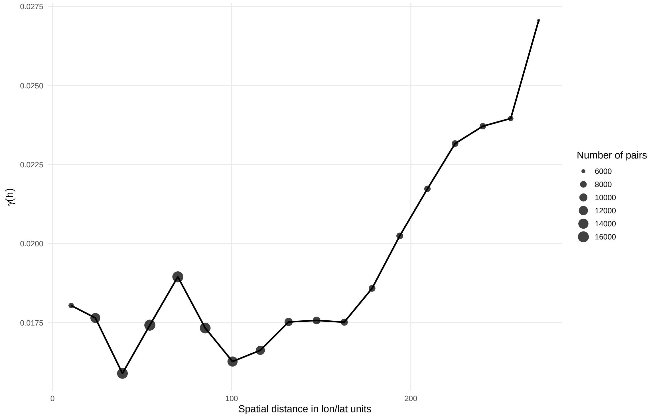
Spatial semivariogram of validation residuals
