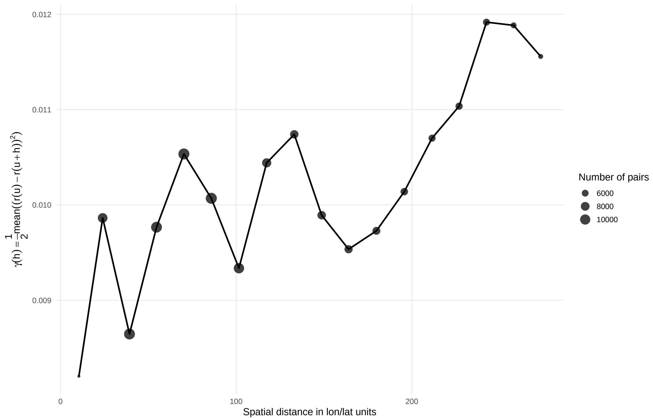
Spatial semivariogram of the mean residual bias
