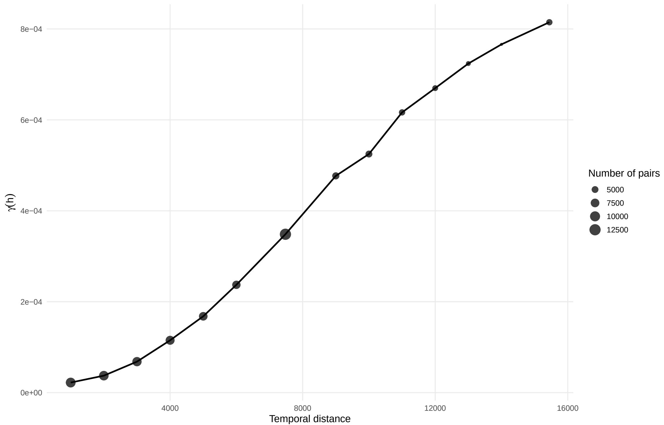
Temporal semivariogram of averaged residuals
