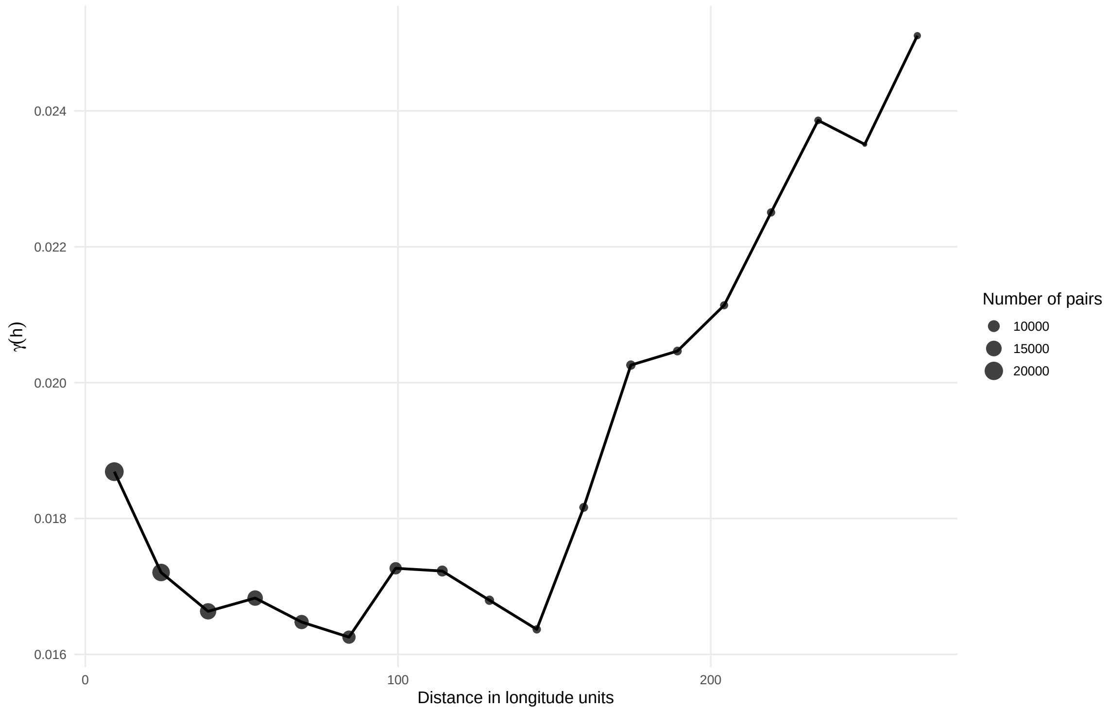
Semivariogram along the longitude direction
