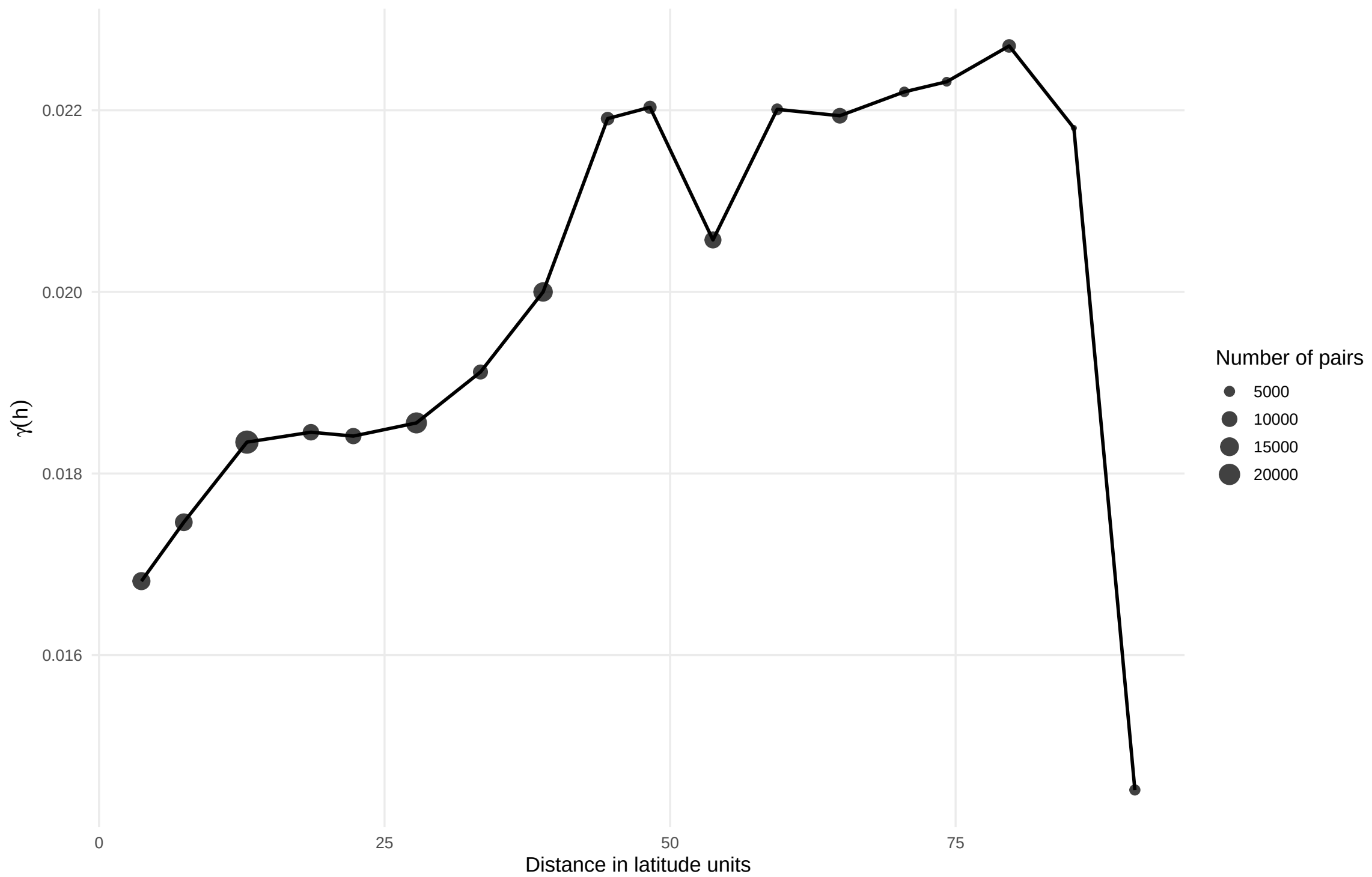
Semivariogram along the latitude direction
