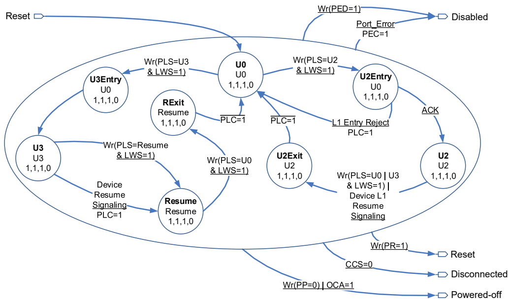
Figure 4-26: USB2 Root Hub Port Enabled Substate Diagram
