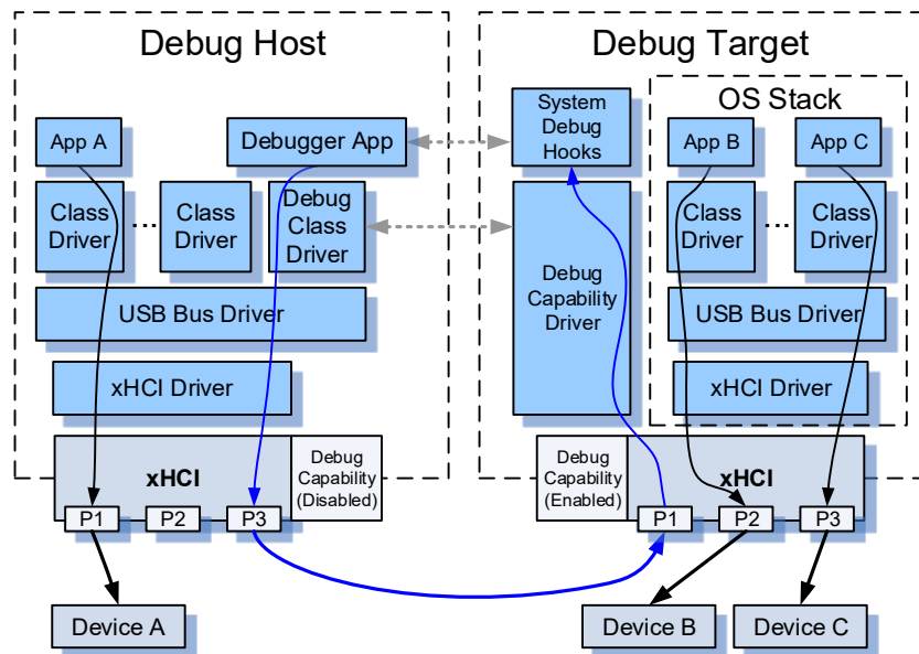
Figure 7-5: Example Debug Software Stacks
