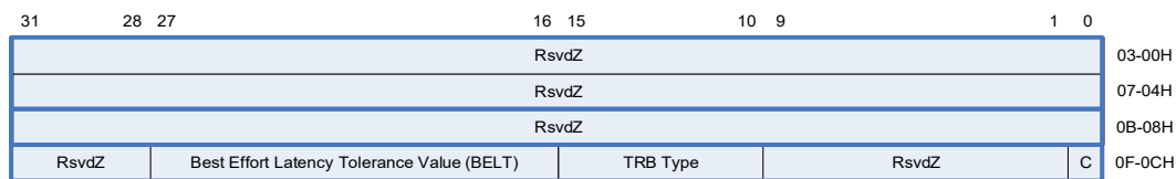
Figure 6-33: Set Latency Tolerance Value Command TRB
