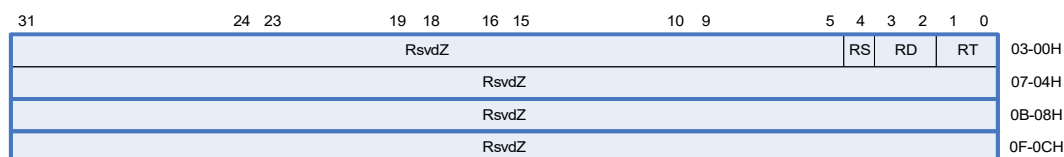
Figure 7-34: Extended Property Context Structure for Get Resource Properties Command
