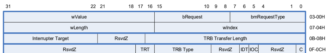
Figure 6-9: Setup Stage TRB
