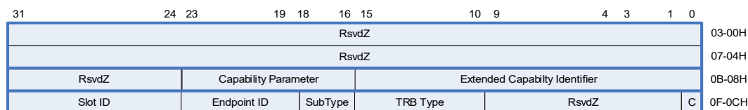
Figure 6-37: Set Extended Property Command TRB
