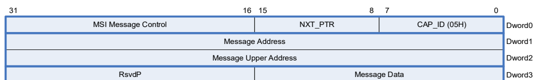
Figure 5-3: PCI MSI Configuration Capability Structure
