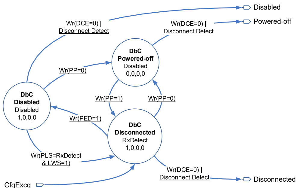
Figure 4-29: USB3 Root Hub Port DbC Substate Diagram
