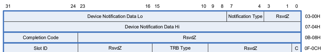
Figure 6-20: Device Notification Event TRB
