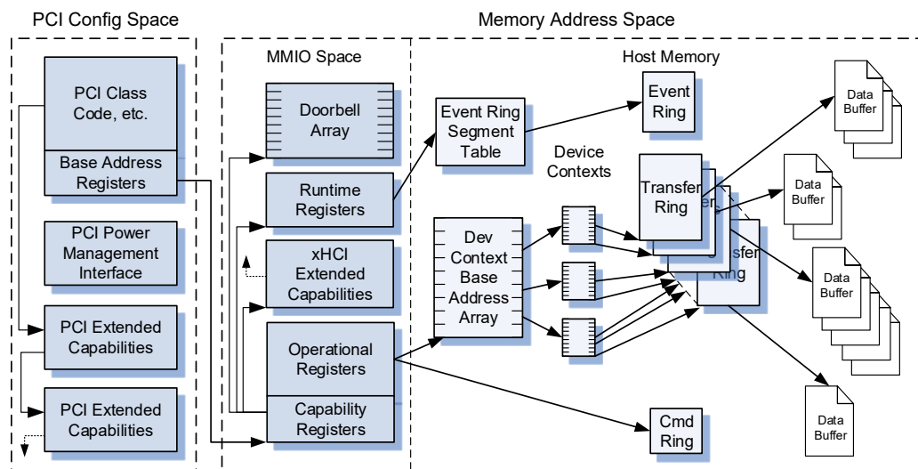
Figure 3-3: General Architecture of the eXtensible Host Controller Interface
