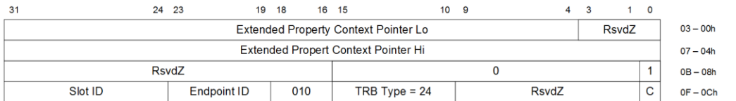
Figure 7-21: Get Endpoint Properties SubType of Get Extended Properties Command
