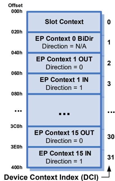
Figure 6-1: Device Context Data Structure
