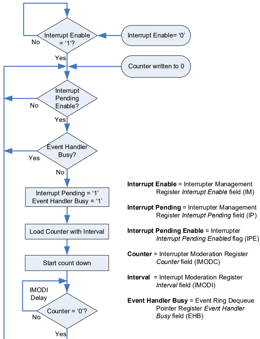
Figure 4-24: Interrupt Throttle Flow Diagram
