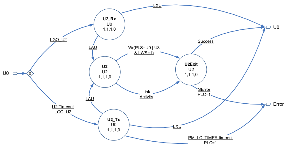
Figure 4-38: Gen T Root Hub Port U2' Substate Diagram
