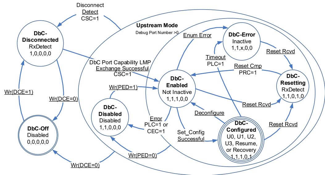
Figure 7-9: DbC Port State Machine
