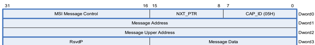
Figure 5-3: PCI MSI Configuration Capability Structure
