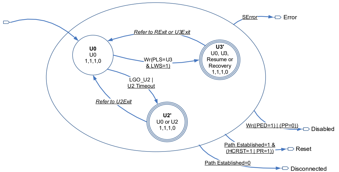
Figure 4-37: Gen T Root Hub Port Enabled Substate Diagram
