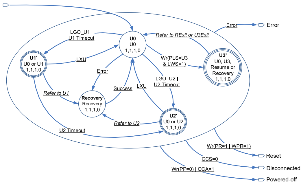
Figure 4-32: USB3 Root Hub Port Enabled Substate Diagram
