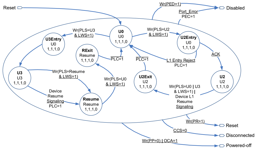
Figure 4-28: USB2 Root Hub Port Enabled Substate Diagram
