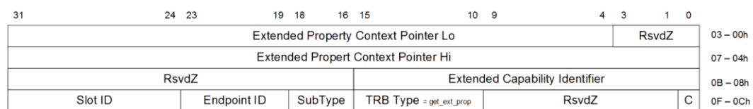
Figure 6-36: Get Extended Property Command TRB
