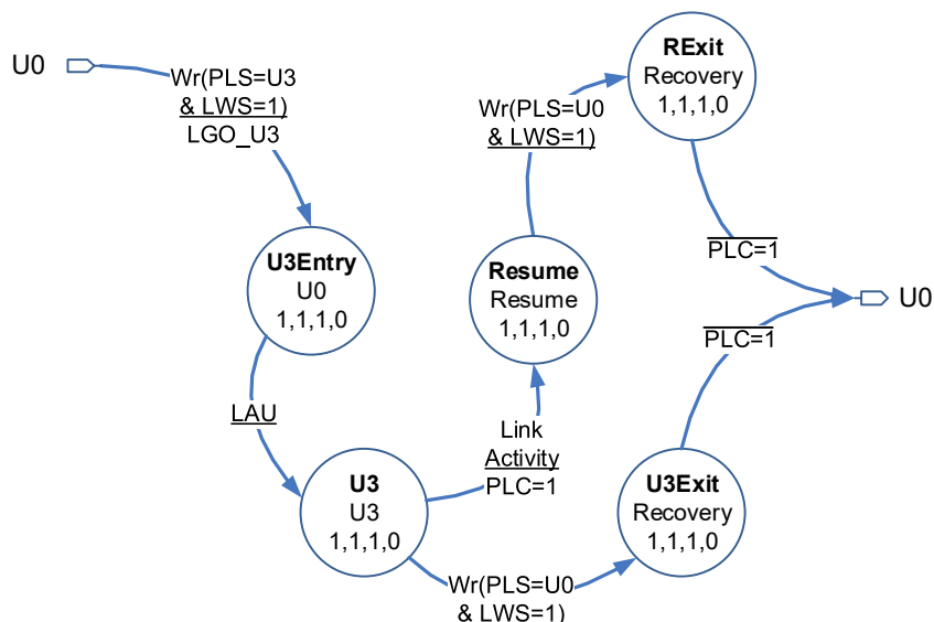
Figure 4-35: USB3 Root Hub Port U3' Substate Diagram
