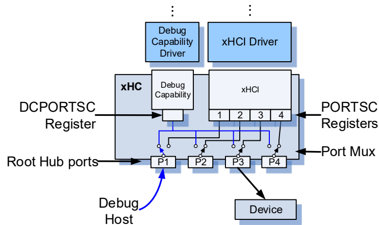
Figure 7-8: Debug Port Multiplexing
