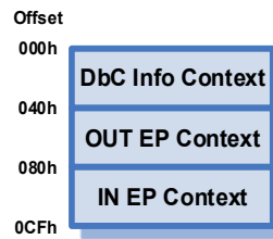
Figure 7-11: Debug Capability Context Data Structure
