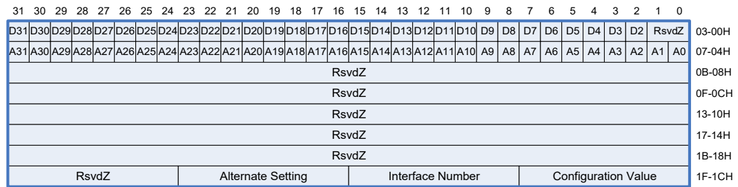
Figure 6-6: Input Control Context
