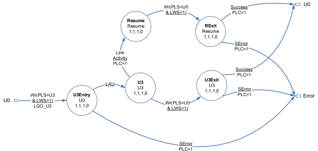
Figure 4-39: Gen T Root Hub Port U3' Substate Diagram
