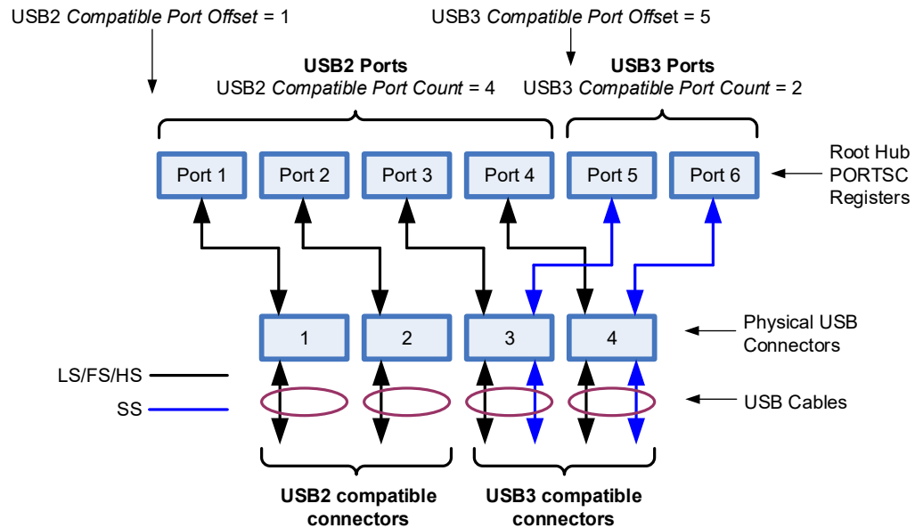
Figure 4-41: Port Routing Example
