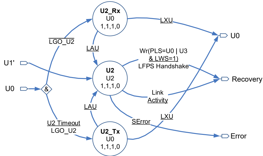
Figure 4-34: USB3 Root Hub Port U2' Substate Diagram
