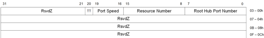
Figure 7-23: Extended Property Context Structure for Get Endpoint Properties Command
