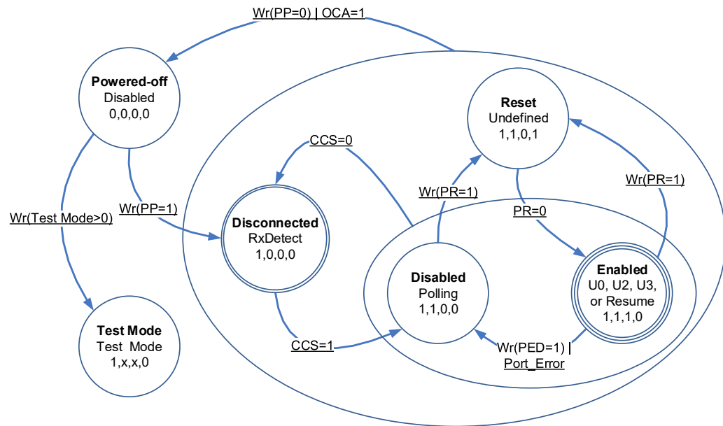
Figure 4-27: USB2 Root Hub Port State Machine
