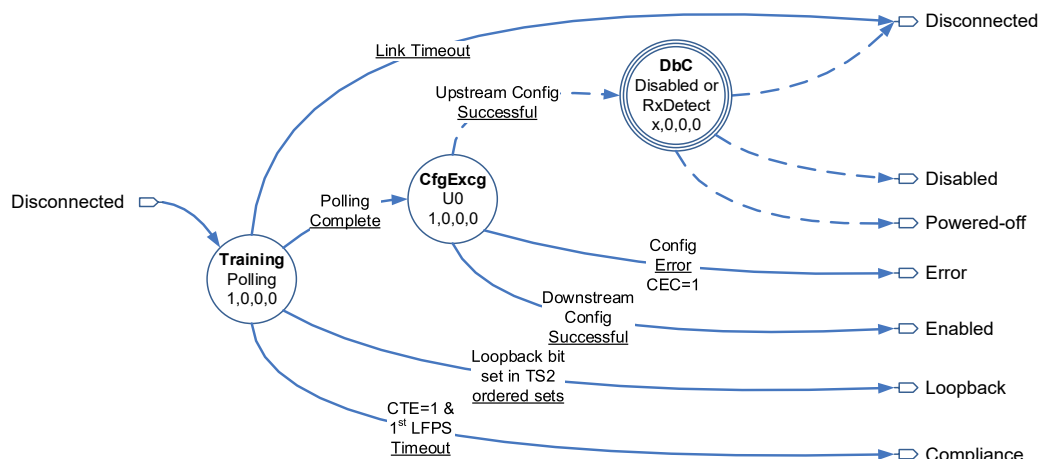
Figure 4-30: USB3 Root Hub Port Polling Substate Diagram
