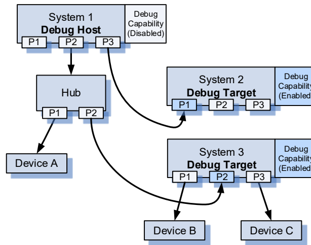
Figure 7-5: Example Debugging Topology
