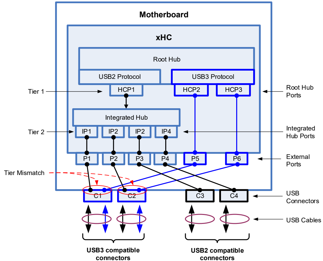
Figure 4-44: Integrated Hub Example
