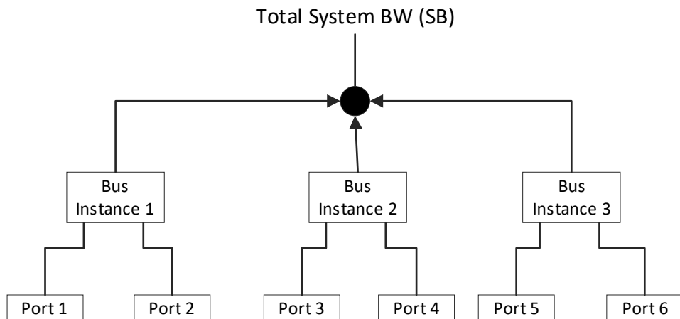
Figure 4-23: Example of an xHC implementation with multiple ports per BI
