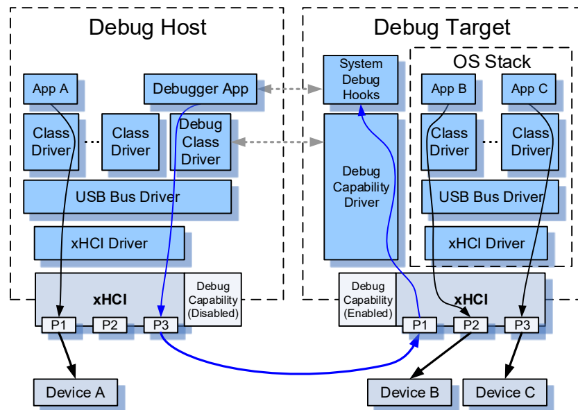
Figure 7-6: Example Debug Software Stacks
