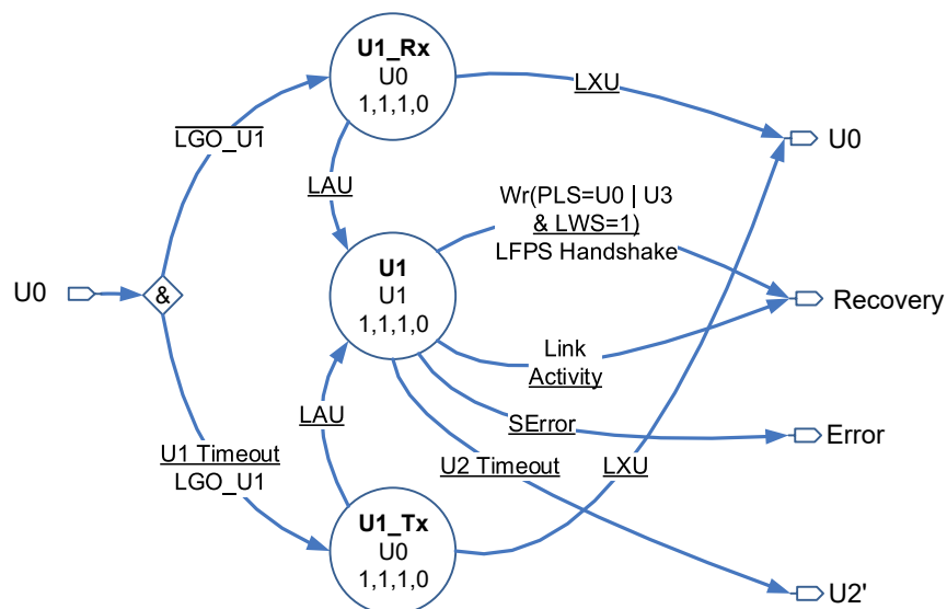
Figure 4-33: USB3 Root Hub Port U1' Substate Diagram
