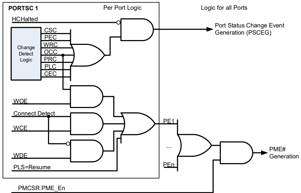
Figure 4-40: Example Port Change Bit Port Status Change Event Generation
