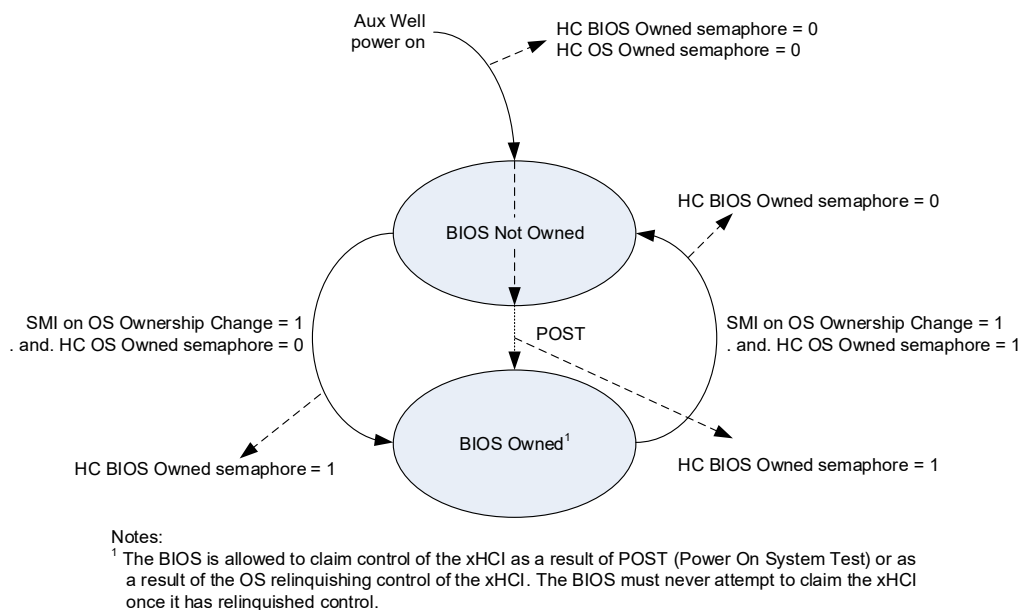
Figure 4-42: BIOS Ownership State Machine
