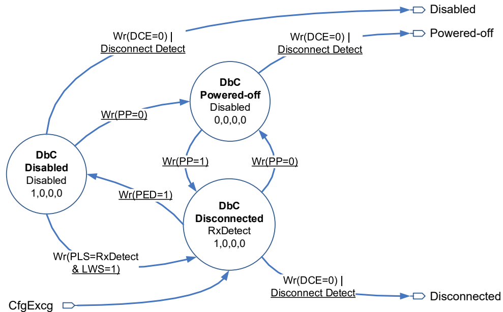
Figure 4-31: USB3 Root Hub Port DbC Substate Diagram
