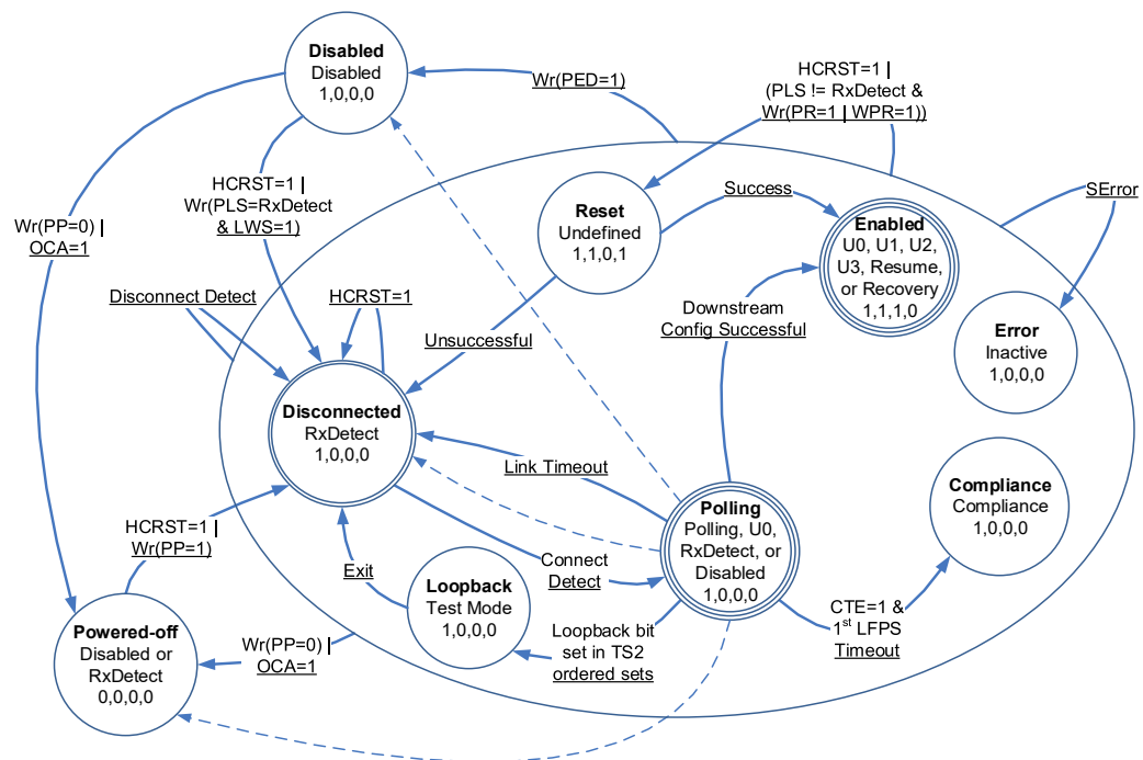
Figure 4-29: USB3 Root Hub Port State Machine
