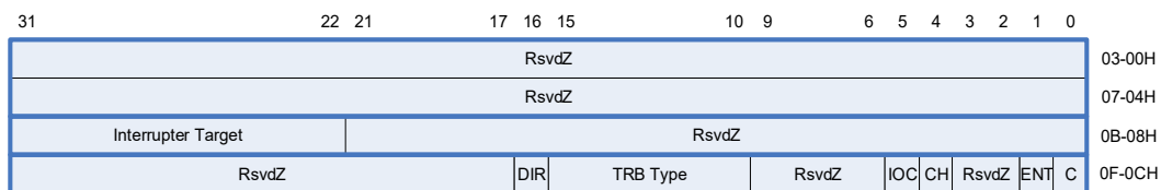
Figure 6-11: Status Stage TRB
