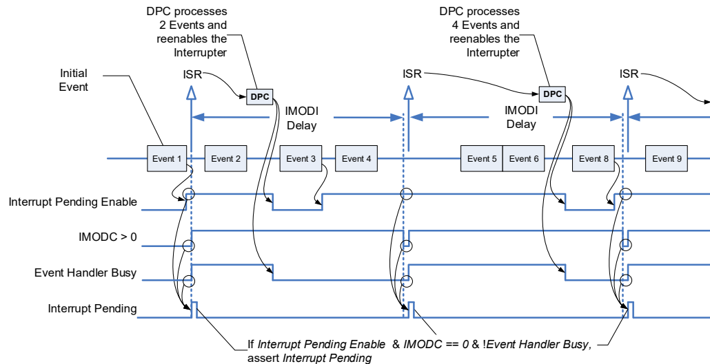
Figure 4-25: Heavy load, interrupts moderated
