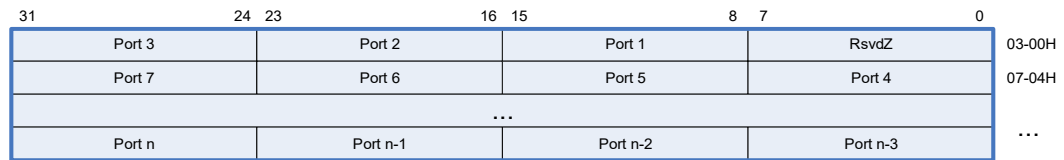
Figure 6-7: Port Bandwidth Context
