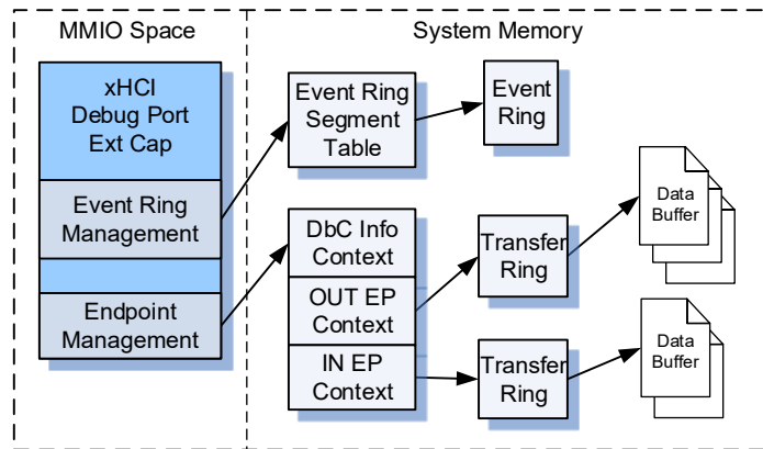
Figure 7-7: Debug Capability Memory Map
