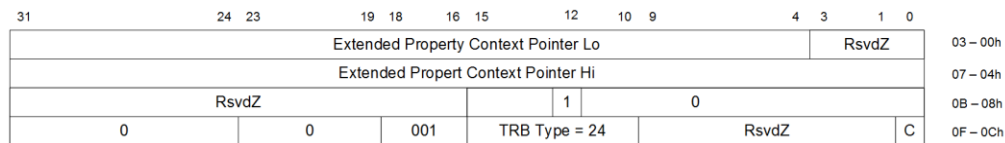
Figure 7-26: Get Time Stamp Command SubType
