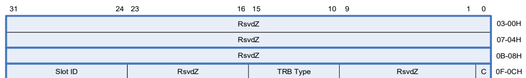
Figure 6-31: Reset Device Command TRB
