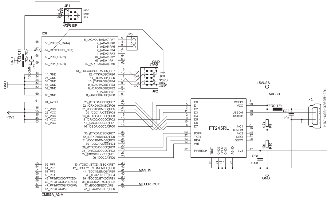
Figure J.1: Schematics of the microcontroller and the USB interface.
