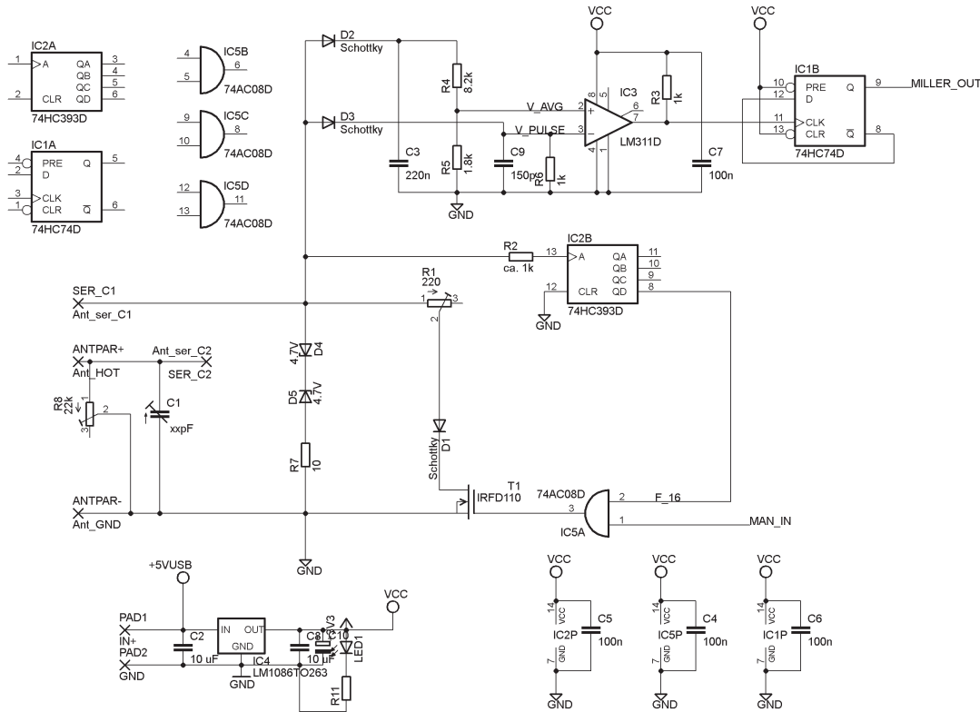
Figure J.2: Circuit diagrams of the power supply and the (de)modulation circuitry of the Chameleon
