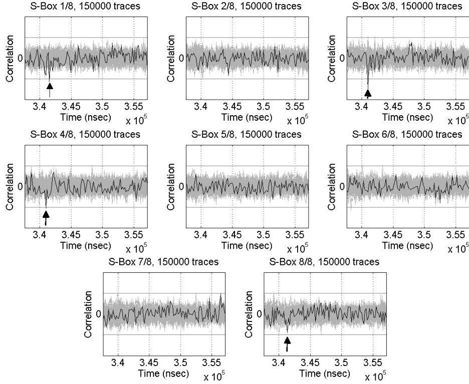
Figure 7.17: First attempt of a bin-wise CPA with peak extraction. The depicted correlation coefficients were computed from 150,000 filtered traces, with f_{\text{lowpass}} = 8 MHz and f_{\text{highpass}} = 50 kHz, and reveal the correct key bits for only some of the S-Boxes.
