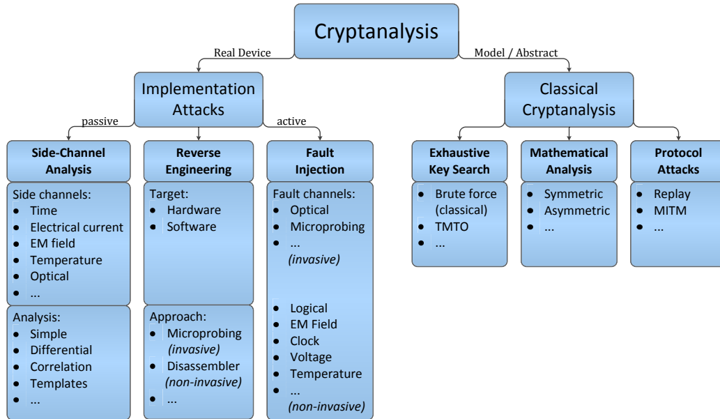
Figure 3.1: Overview of the field of cryptanalysis
