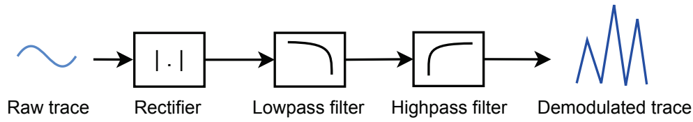
Figure 7.12: Block diagram of incoherent digital amplitude demodulator.
