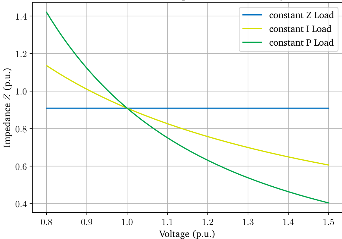
Characterization Impedance Z vs. Voltage
