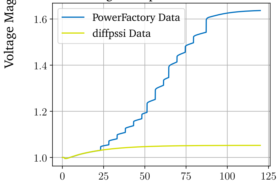
Voltage Comparison for Bus 2
