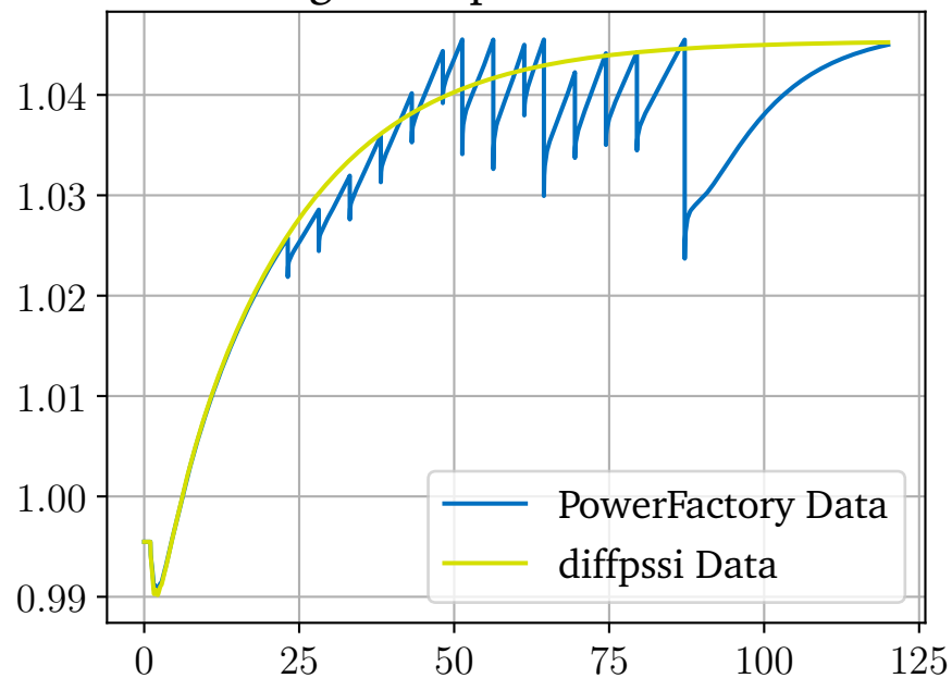
Voltage Comparison for Bus 1
