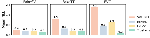
Figure 5: Proper scoring rule risk. Lower NLL values indicate higher trustworthiness with fewer overconfident errors.
