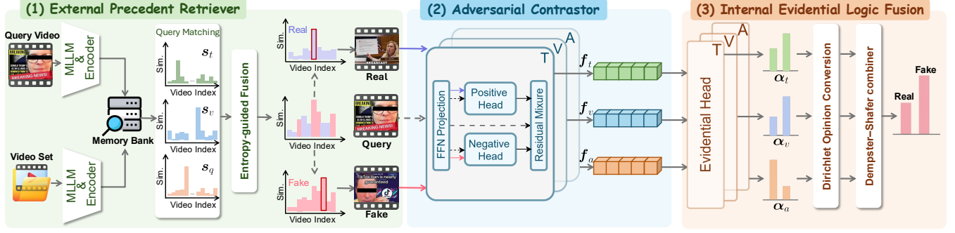
Figure 2: Overview of the proposed method, TrueLens. (1) External Precedent Retriever first decomposes the query video q as three sub-queries, i.e., text, visual and audio queries, while enhancing the text query with the theme and storyline extracted by the MLLM. To fuse different ranking lists by modality-specific query, we introduce an entropy-aware weighting mechanism. Finally, we sort the fused similarity and obtain the most relevant video reference pairs from both real and fake video galleries (i.e., one real and one fake) as external evidence; (2) Adversarial Contrastor considers the positive context of the original query and real query via the positive head, while fusing the original query with fake video via the negative head. Then we jointly take the positive and negative context into consideration, and output modality-specific internal representations through contrastive attention heads; (3) Internal Evidential Logic Fusion first models internal modality-specific evidence separately via independent evidential heads, and then integrates them using a theoretically guaranteed rule to produce trustworthy final predictions.
