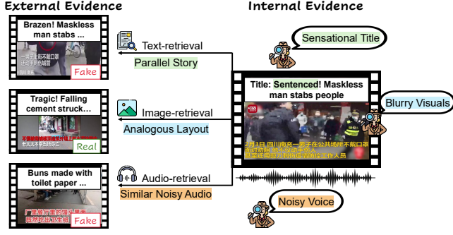
Figure 1: Motivation of our work. We argue that external and internal evidence are complementary for video fake news detection, facilitating contextual reasoning. Left: External evidence is obtained by leveraging the video’s multimodal content (text, image, audio) as queries to retrieve related video references. Right: Internal evidence is mined from intrinsic cues within the video itself, such as sensationalist text, visual artifacts (e.g., low quality), and audio distortions (e.g., noisy speech).
