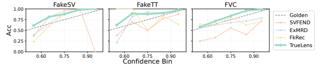
Figure 4: Calibration diagram. Curves closer to the golden dashed line indicate better calibration.
