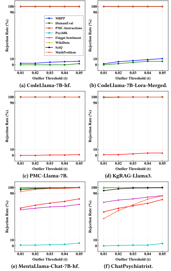
Figure 5: Ablation results based on outlier thresholds ( t ).
