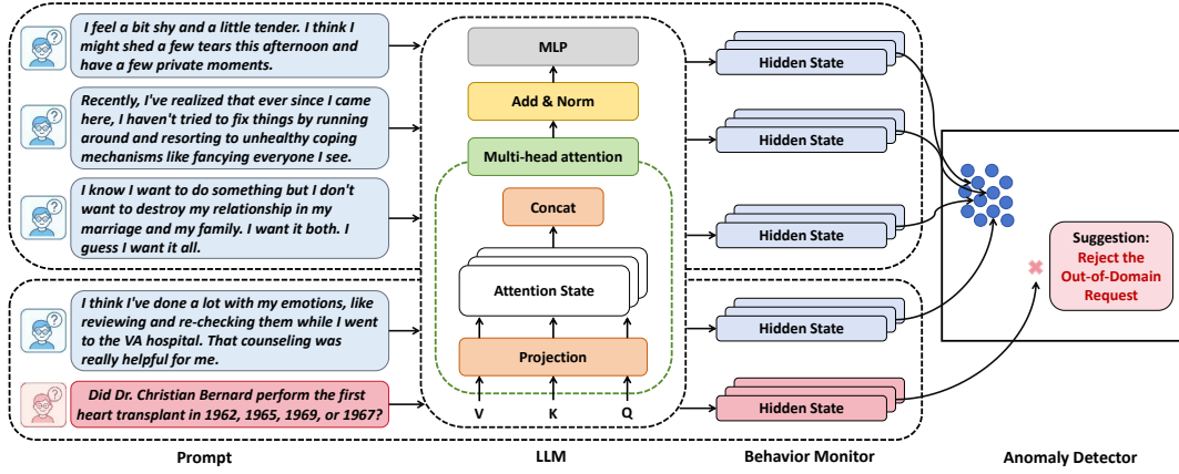
Figure 2: Overall framework of DomainMonitor.
