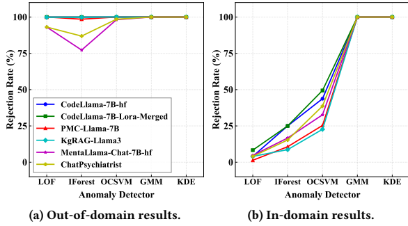
Figure 7: Ablation results on anomaly detectors.
