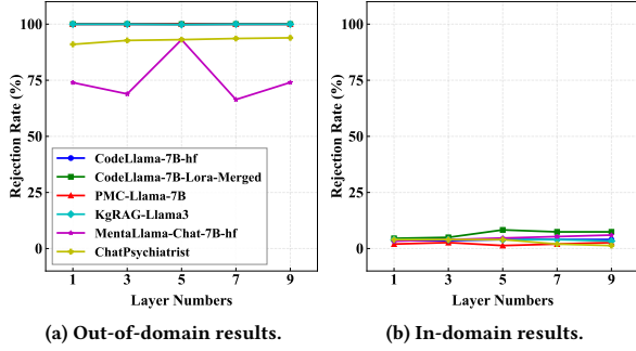
Figure 6: Ablation results on hidden state layers.
