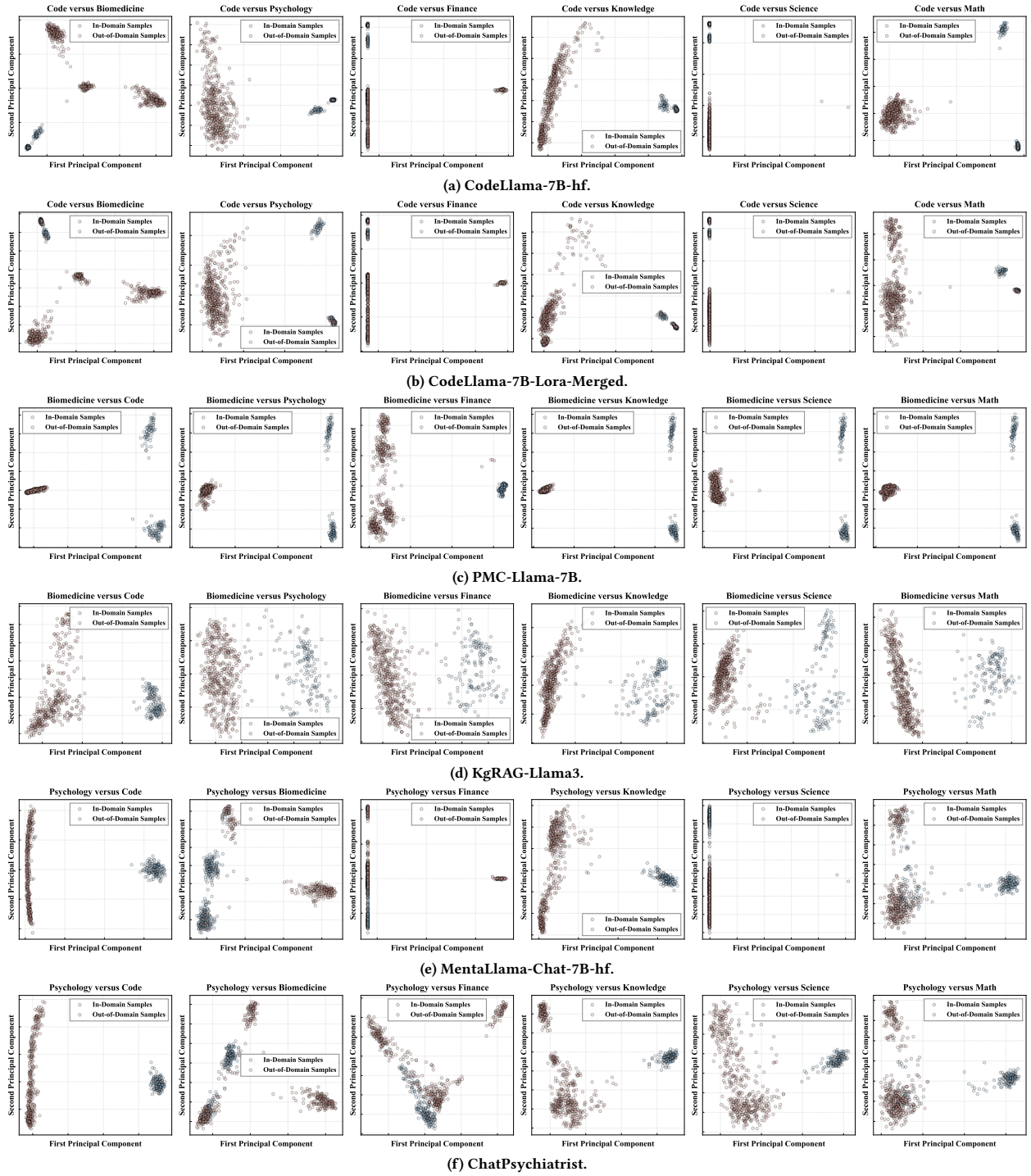
Figure 3: Visualization of LLM hidden states.
