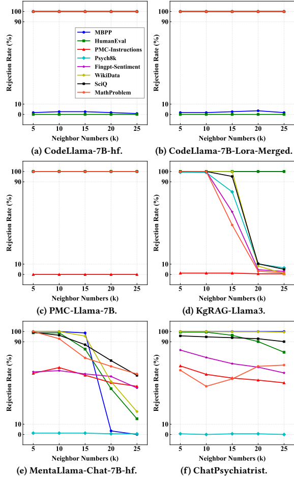
Figure 4: Ablation results based on neighbor numbers ( k ).
